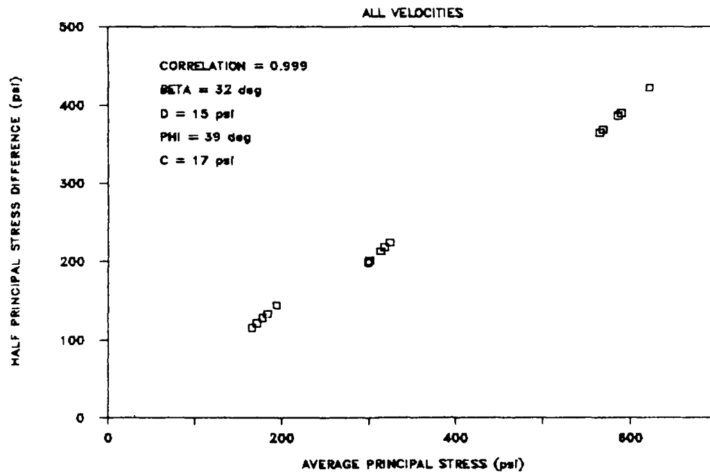
Figure 3.30, STRENGTH ENVELOPES
