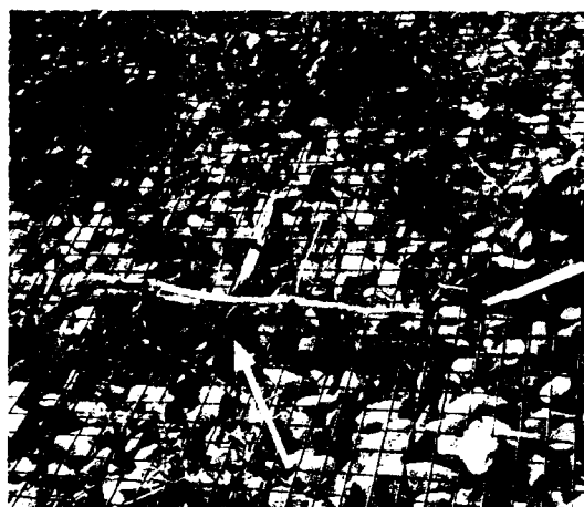
Wire mesh over stone. Note "rebar staple" driven through mesh into the bank
