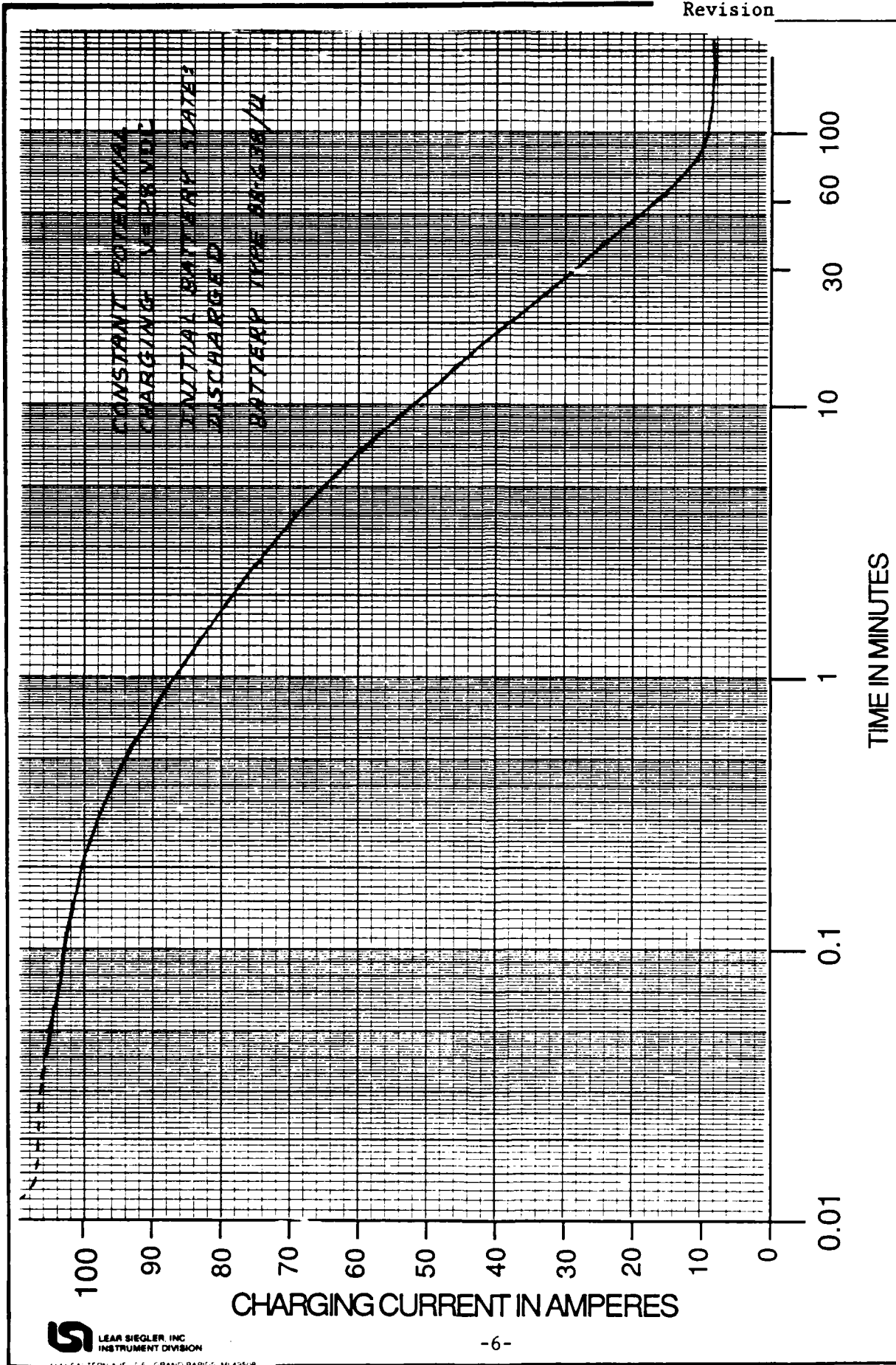
Figure 2. Battery Charge Curve
