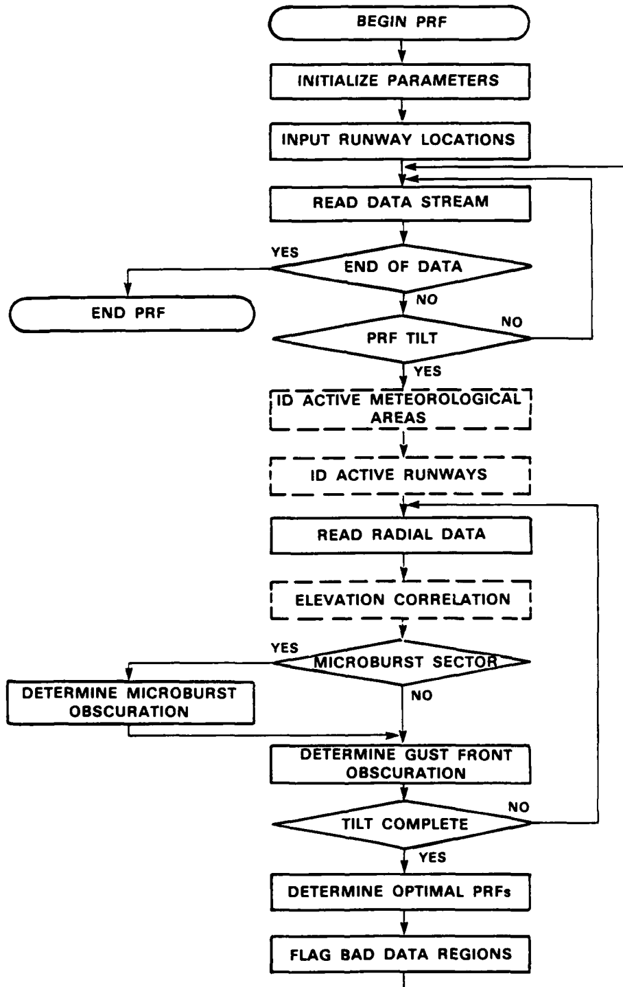
Figure 4-1. Top level flow diagram for PRF algorithm.
