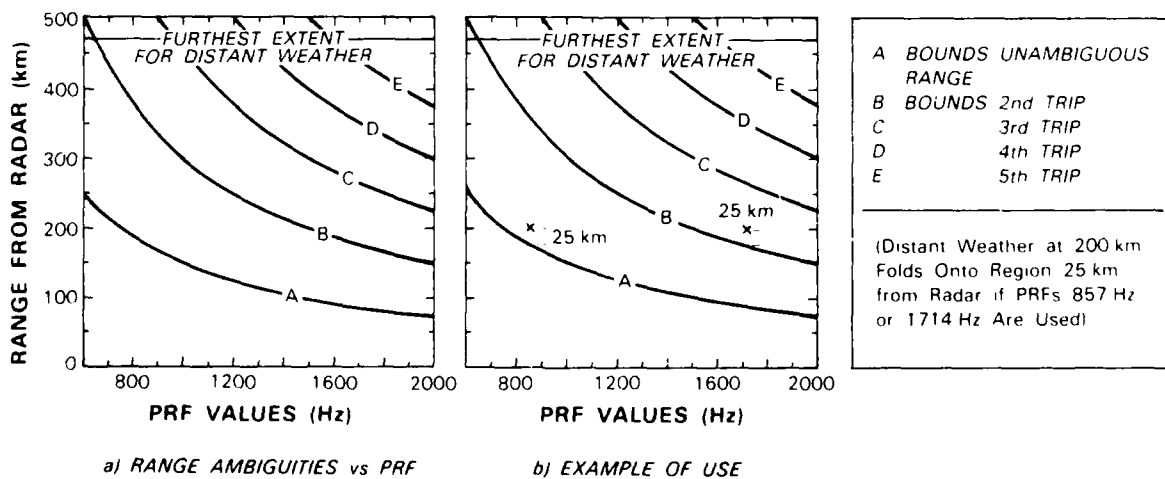
Figure 2-1. Obscuration vs PRF value.
