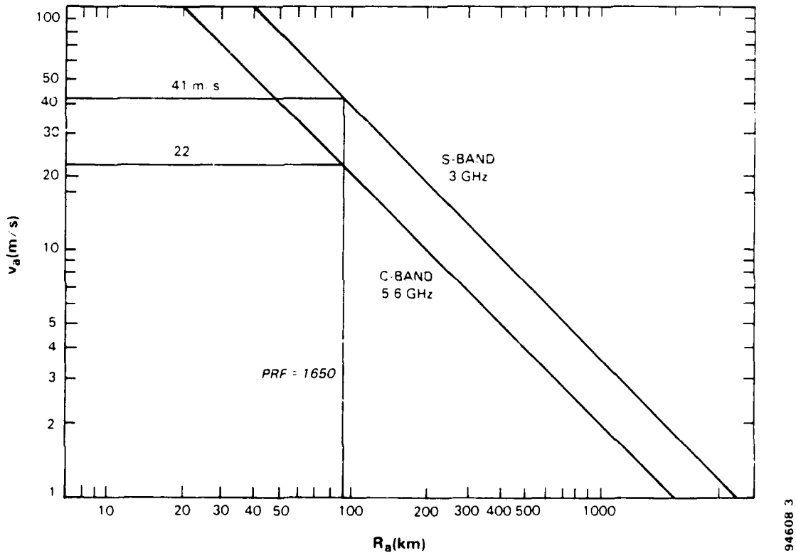
Figure 1-2. Simultaneous unambiguous R_a and v_a intervals.
