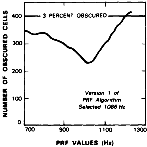
Figure 4-4. Gust front obscuration profile at 0107 UT.
