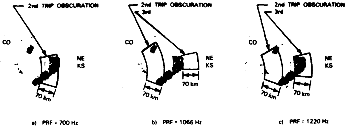
Figure 4-3. Obscuration assessment at 0107 UT.
