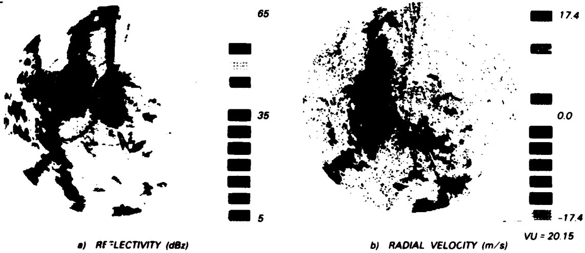
Figure 4-22. Range aliased returns at 2023 UT.
