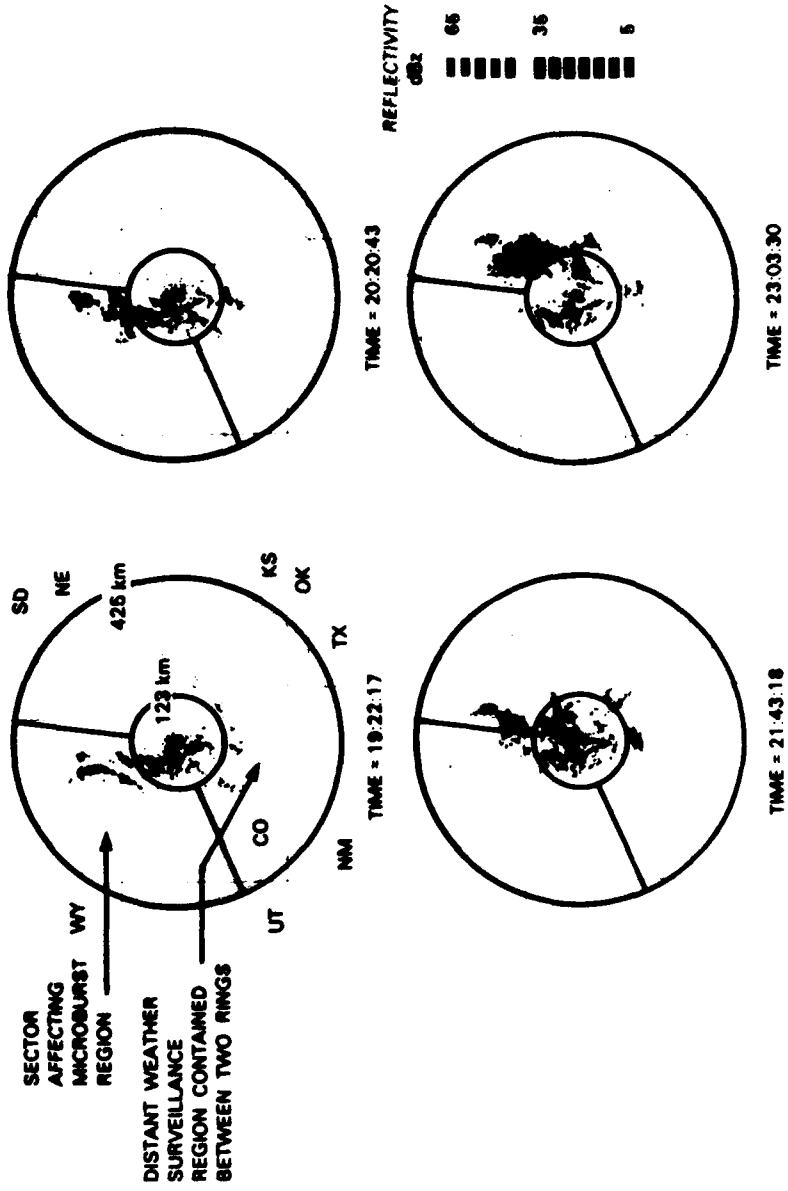
Figure 4-15. Reflectivity profiles of 4 September 1987.
