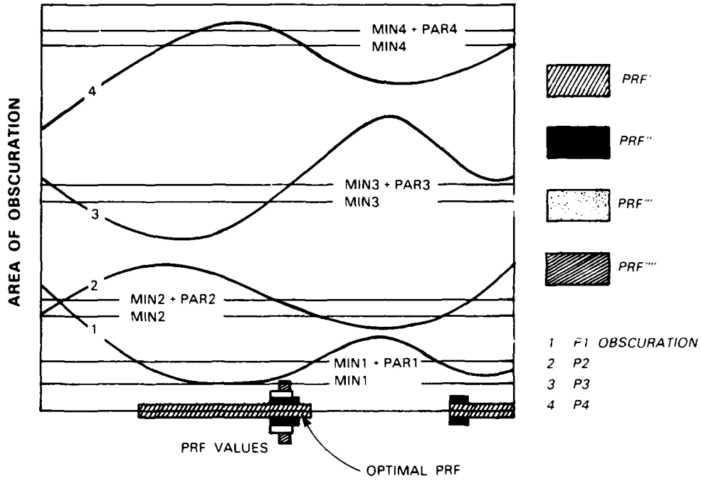
Figure 3-1. An example of the PRF selection criteria.
