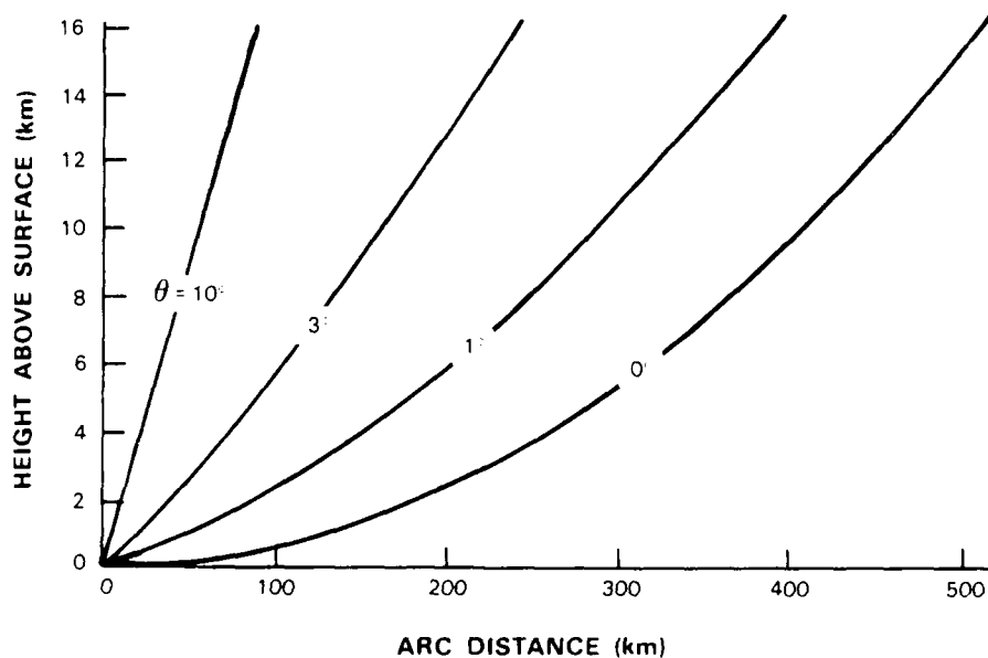
Figure A-1. Arc distance vs altitude.
