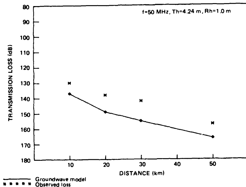
Figure 22. Ohio hills median observed transmission-loss data compared to the GROUNDWAVE model as a function of distance, f=50 MHz, T_h=4.24 m, R_h=1.0 m.
