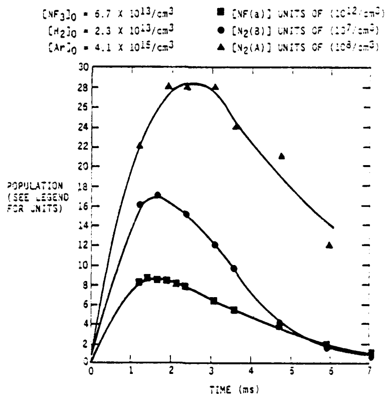
Figure 8. Temporal profiles of NF(a) , N_2(A) , and N_2(B) .
