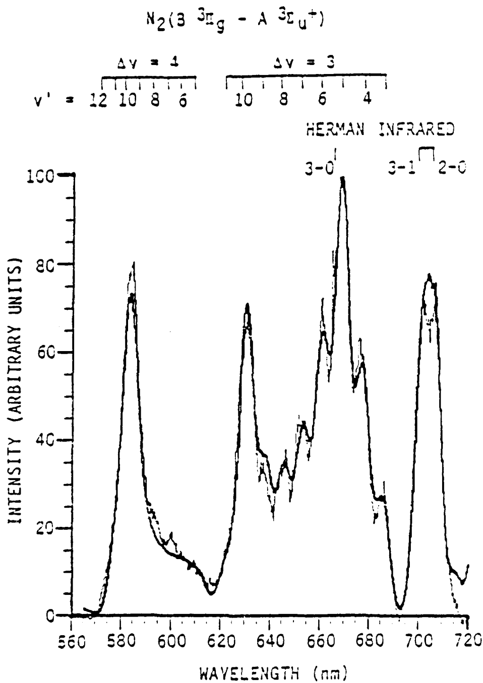
Figure 73. Variation in N_2(3, A) spectrum produced in N_2(A) energy - pooling with changes in nitrogen and argon partial pressures.
