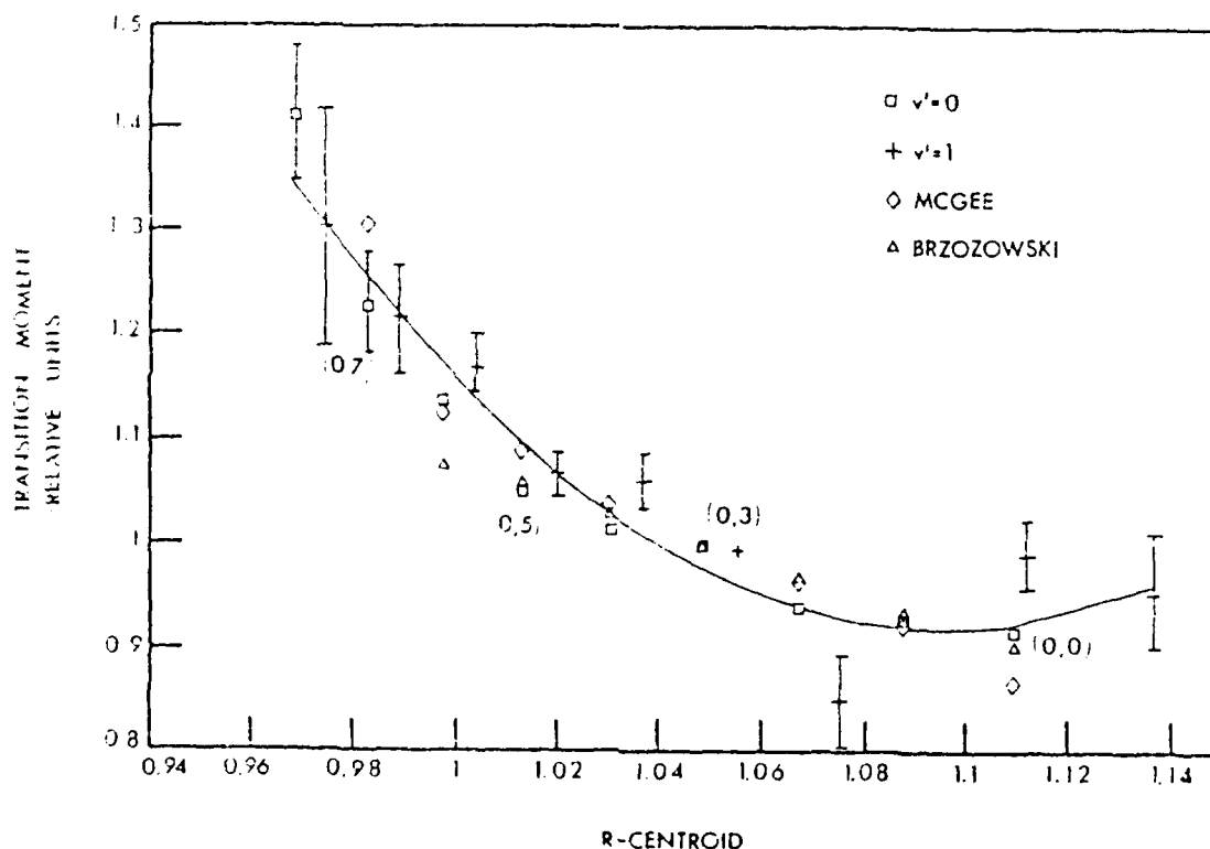
Figure 33. Variation in electronic transition moment with r -centroid for the NO(A-1+ - X2+2) transition.
