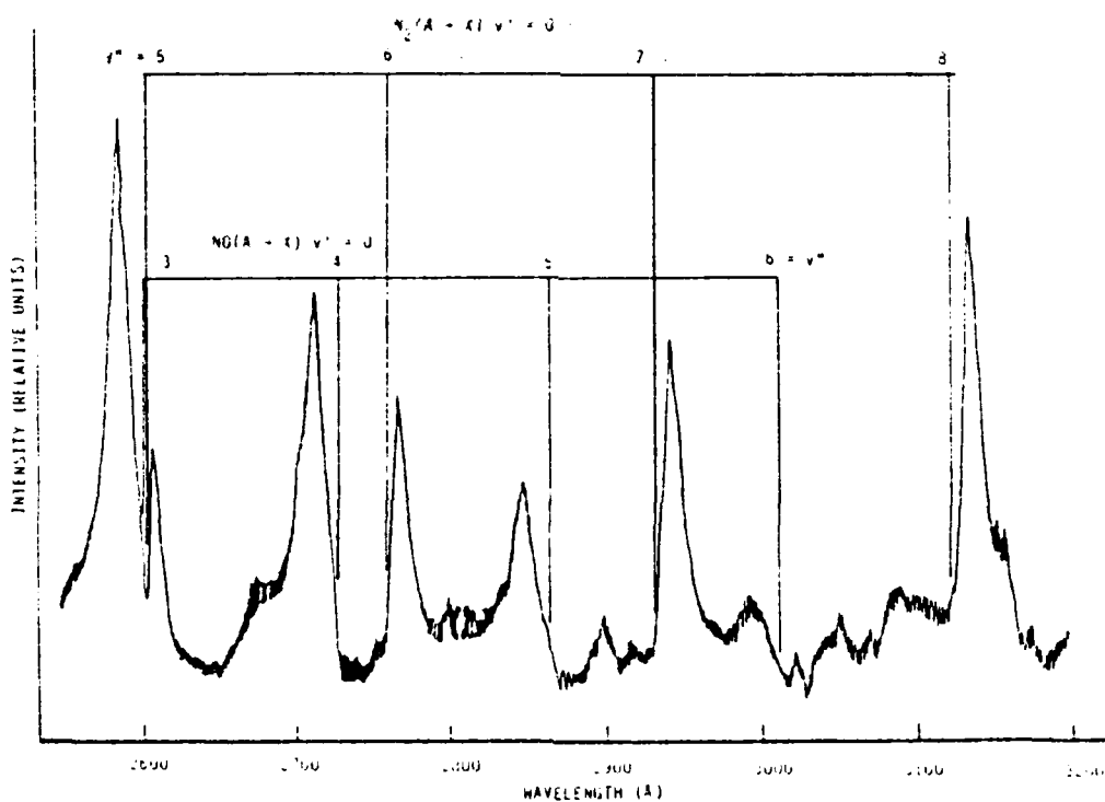
Figure 6. \text{NO}(A+X) and \text{N}_2(A+X) system produced by reacting \text{H}_2 + discharged \text{NF}_3 .
