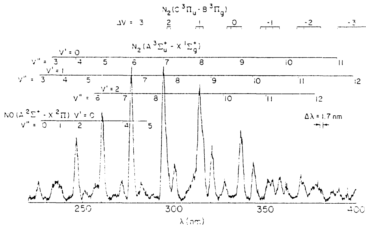
Figure 32. Vegard-Kaplan emission in flow reactor 9 ms downstream from the discharge.
