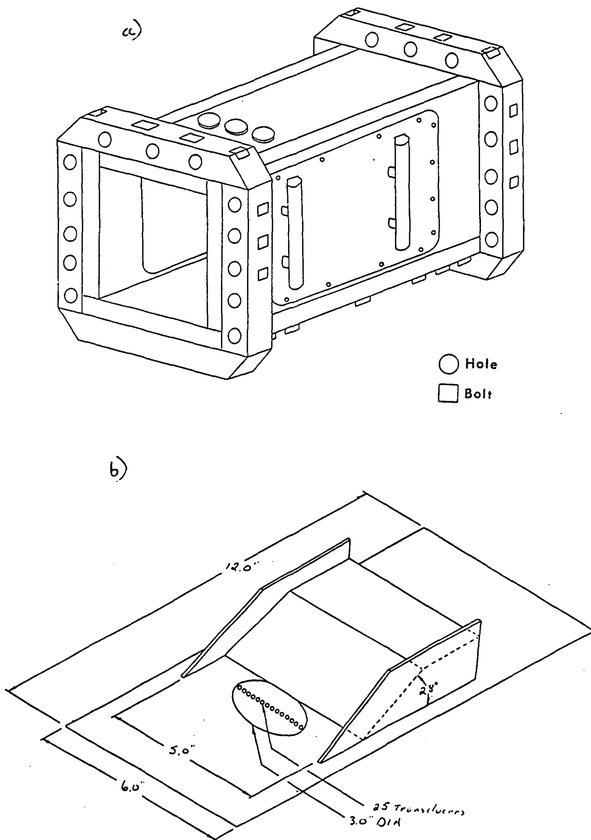
Fig. 1 Test Section and Model
