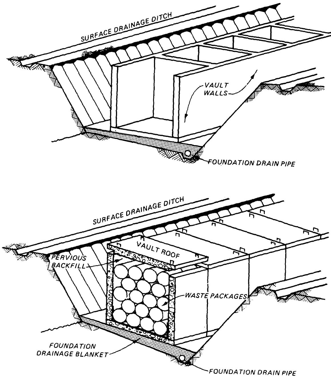
Figure 2.4.3. Top loading concept of waste emplacement in an EMCB
