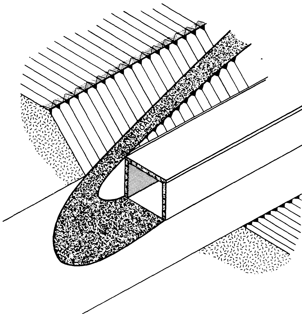
Figure 2.4.2. Side loading concept of waste emplacement in an EMCB
