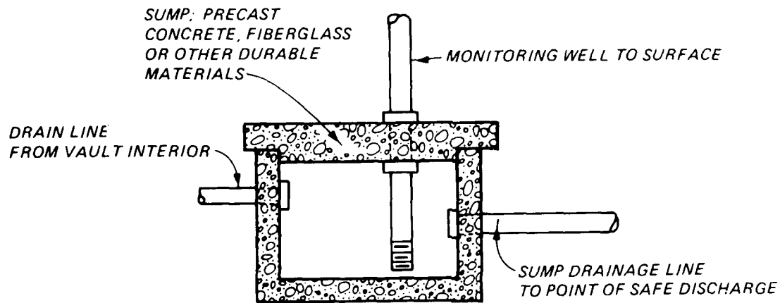
(a) Section view of collector sump for interior drain system
