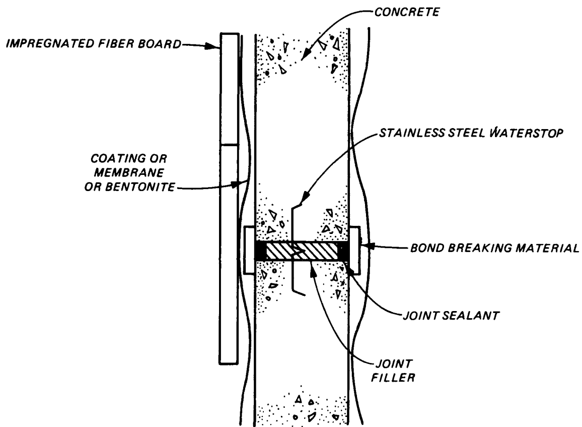
Figure 2.3.1. Moisture barriers for concrete
