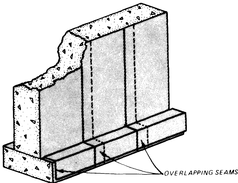
Figure 2.3.2 Low-permeability membranes applied with overlapping seams
