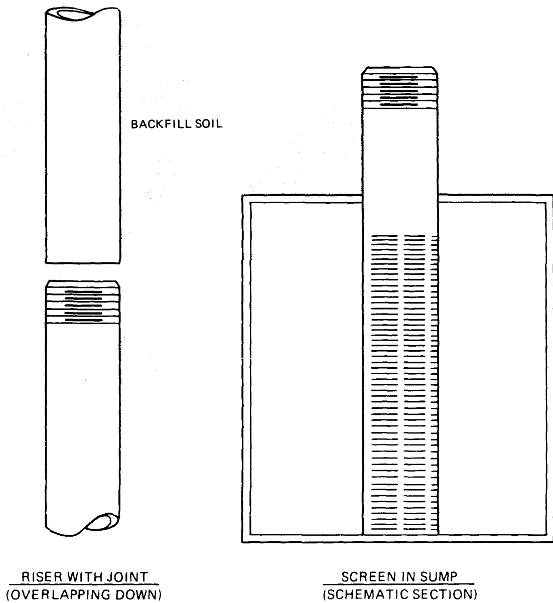
Figure 2.6.1. Features of sump monitoring wells
