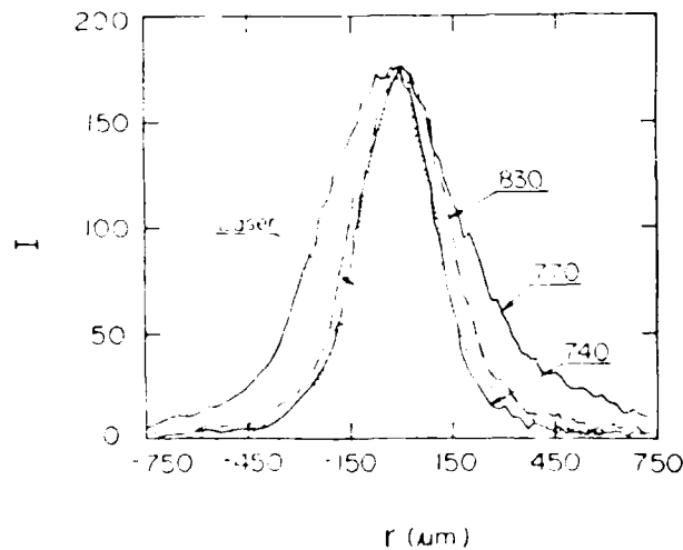
Fig. 12 Time-resolved photoluminescence intensity as a function of position for the device. The curves are photoluminescence from the asymmetric well structure at various wavelengths at 4K.
