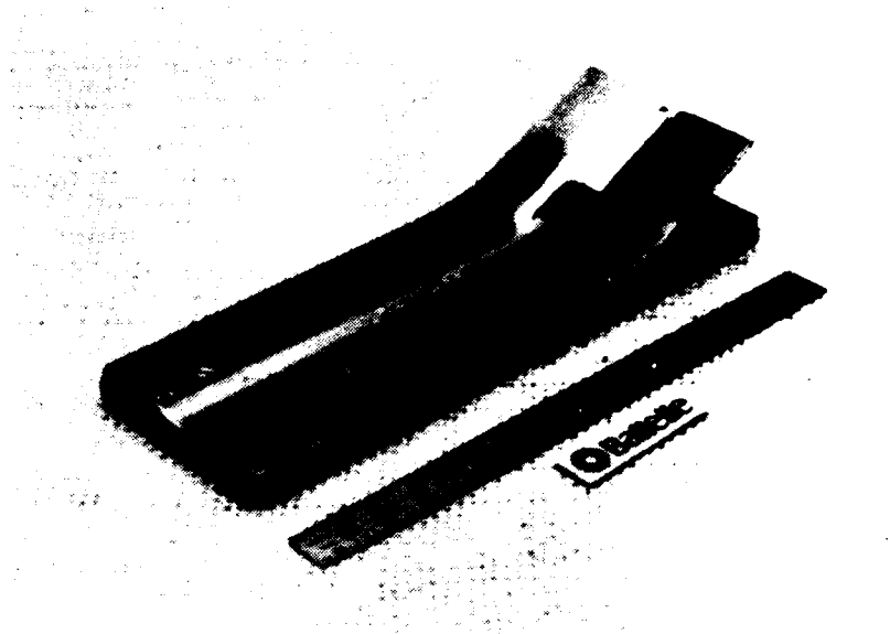
Figure 1. Linear strip weld made with optimum explosive welding conditions.
