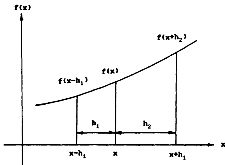
Figure 1.3 Nonuniform mesh.
