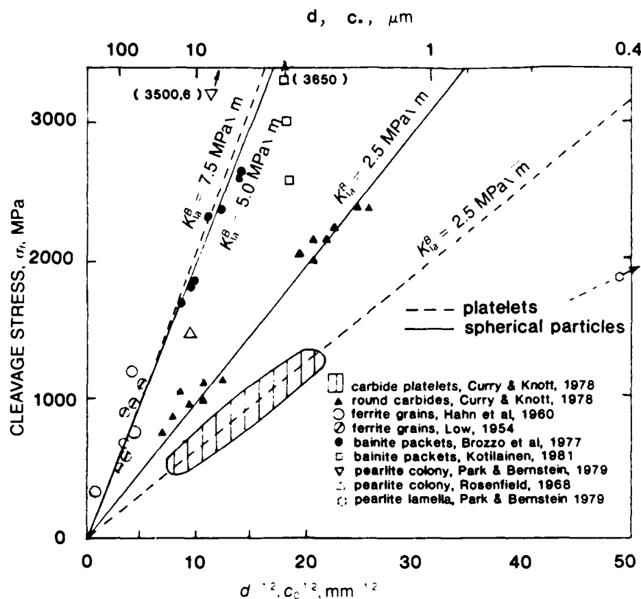
Fig. 8—Summary of brittle fracture stress-particle dimension measurements for different microstructures, showing the characteristic values of K_{IC} . Refs. 9-11, 19, 24, 26-28
