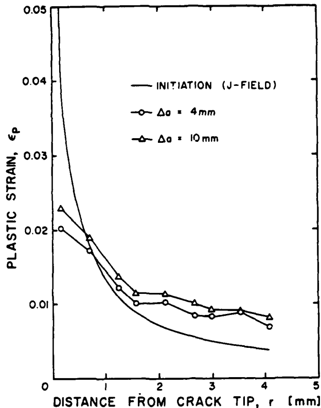
Fig. 14. Plastic strain along a line at 45^\circ to the propagation crack tip.
