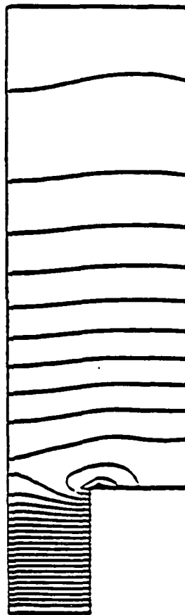
FIGURE 3.b : Pipe flow problem. Stream function and Pressure
