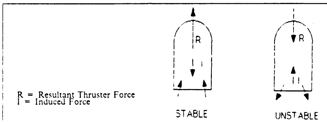
Figure 4.12 Cambered Thruster Instability.
