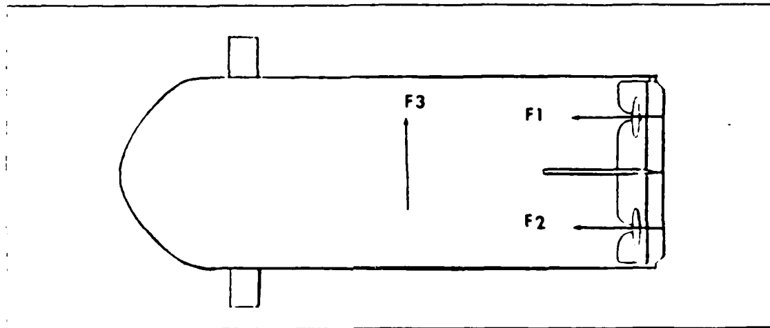
Figure 4.1 Thruster Configuration.
