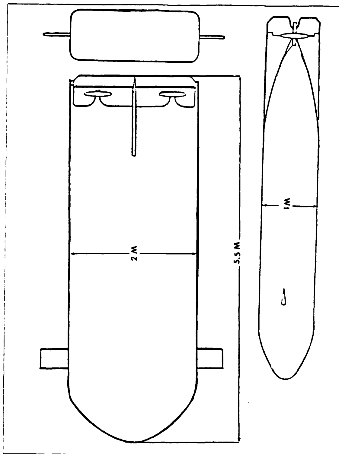
Figure 1.2 AUV Dimensions.
