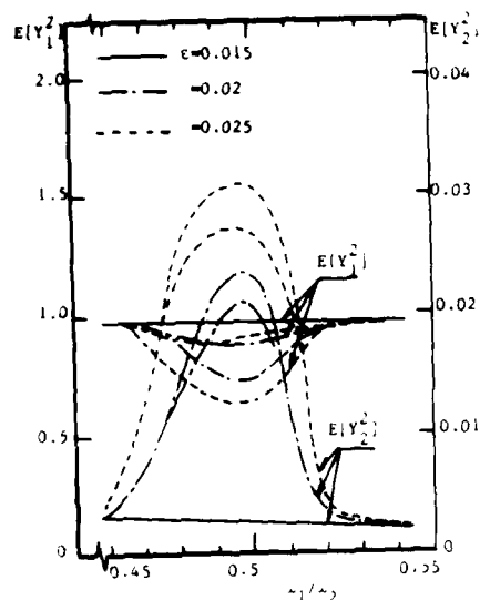
Fig. (2) Gaussian closure solution for various values of nonlinear coupling parameter \epsilon
