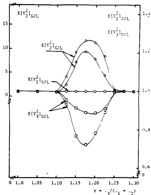
Fig. 15. Mean square response of normalized coordinates as function of internal resonance ratio r , for \zeta_1 = 0.01 , \varepsilon = 0.05
