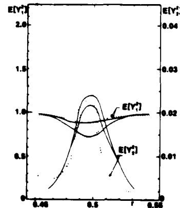
Fig. 4 Mean-square response of normal modes according to Gaussian closure solution vs internal resonance: —, deterministic system; ---, system with random damping, D_{r1} = D_{r2} = 0.1D_0 , 2D_0 = 0.02 .
