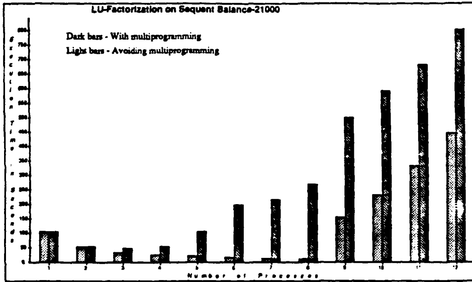
Figure(3) LU-Factorization on Sequent's Balance-21000 using Barriers
