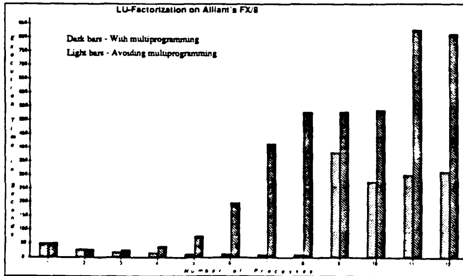
Figure(2) LU-Factorization on Alliant's FX/8 using Barriers
