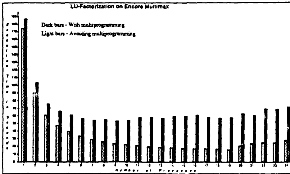
Figure(4) LU-Factorization on Encore's Multimax using the new method
