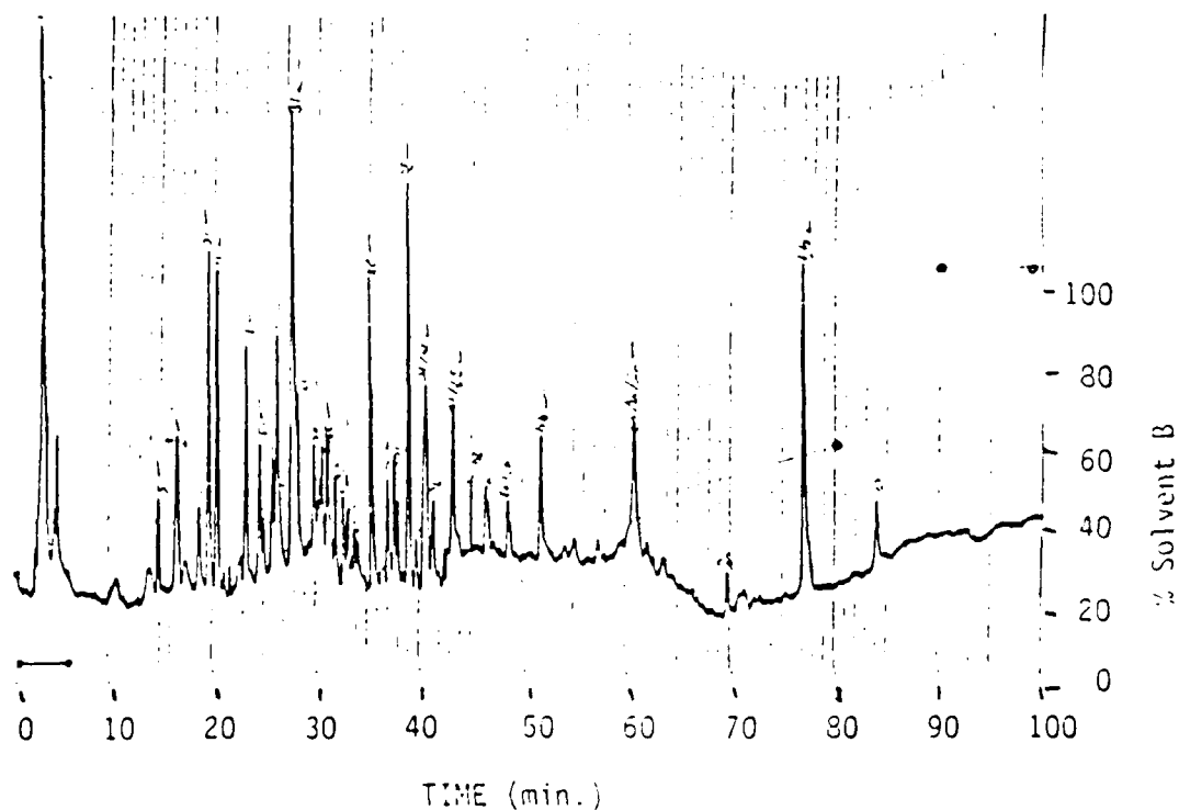
Figure 5: Preparation of chymotryptic peptides of AChE. AChE (150 \mu\text{gm} in 350 \mu\text{l} 100 mM sodium phosphate, pH 8.0 containing 0.5 percent octylglucoside) was treated at 37°C for 2 h with 3 \mu\text{gm} of chymotrypsin. The peptides generated were separated on a C4 Vydac reverse phase column as described for tryptic peptides.
