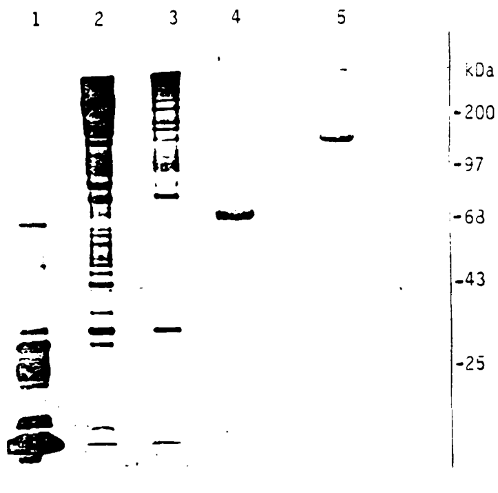
Figure 2: SDS-PAGE analysis of AChE purification. Lane 1, hemolysate, 60 \mu g; lane 2, red blood cell ghosts, 10 \mu g; lane 3, 100,000 xg supernatant, 3 \mu g; lane 4, affinity purified AChE, 1.5 \mu g after disulfide reduction; lane 5, affinity purified AChE, 1.5 \mu g protein, without disulfide reduction. The protein bands were visualized by silver staining. M_r standards are myosin heavy chain, 200 kDa; phosphorylase b, 97 kDa; bovine serum albumin, 68 kDa; ovalbumin, 43 kDa; chymotrypsinogen, 25 kDa.
