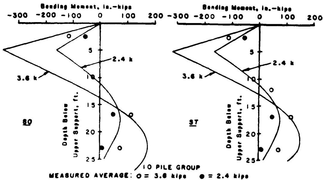
Fig. 9.28 Predicted Moment vs. Depth, Harvey Test, Cyclic
