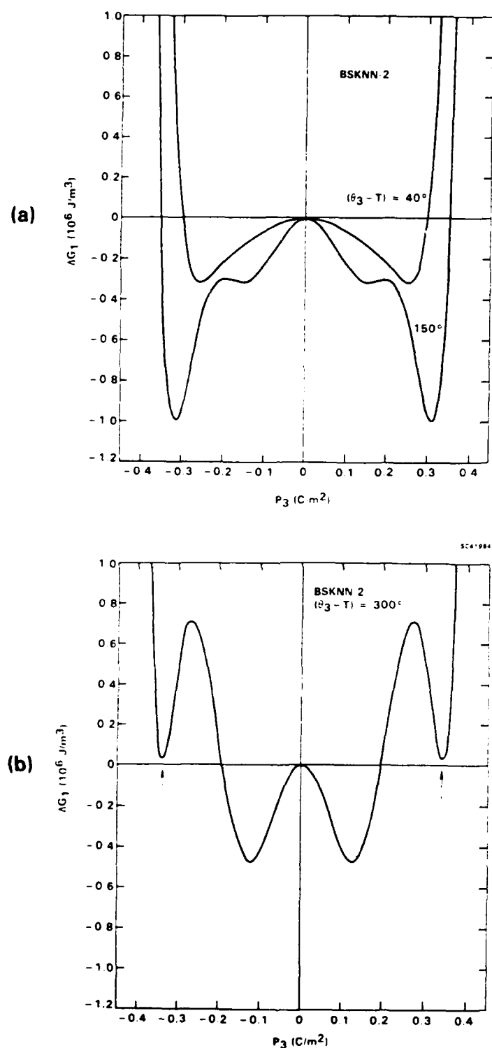
Fig. 7 (a) Calculated Gibbs free energy curves for BSKNN-2 at ( \theta_3 - T ) = 40° and 150°C, showing absolutely stable ferroelectric states at the energy minima P_3 = \pm P_s . (b) Calculated Gibbs free energy curve for BSKNN-2 at ( \theta_3 - T ) = 300°C, showing metastable ferroelectric states at P_3 = \pm P_s .
