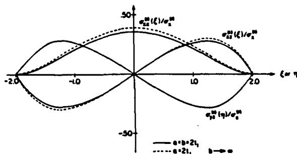
Fig. 3 \sigma_{xx}^{(1)} , \sigma_{xx}^{(2)} , and \sigma_{yz}^{(1)} variation
