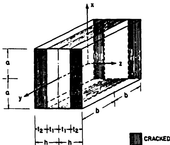
Fig. 2 Repeating element
