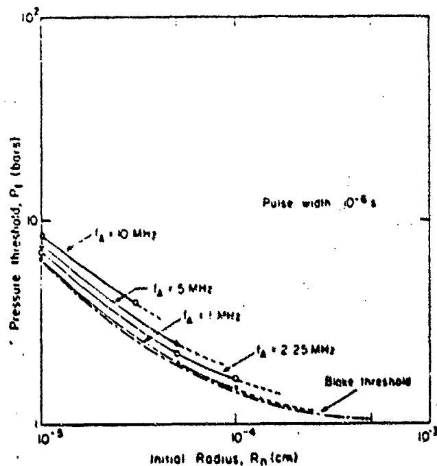
Figure 2.3 Threshold Pressure P_t (in Bars) for Transient Cavitation as a Function of Initial Radius R_0 Over a Range of Frequency f_A at a Pulse Width of 1\mu s [Ref. 4]
