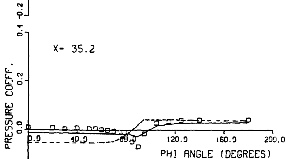
Figure 40. Cp vs. Phi Angle Comparisons, M = 2.0 (Continued)
