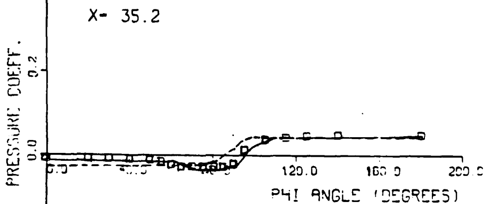
Figure 41. Cp vs. Phi Angle Comparisons, M = 5.0 (Continued)
