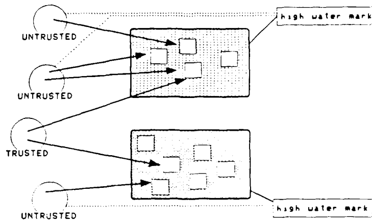
Fig10.2: Objects accessed by untrusted software all have the same high water mark.
