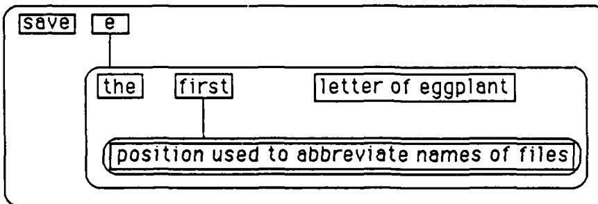
Figure 1b: A nested interpreted structure.
