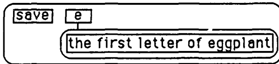
Figure 1a: An interpreted structure shown diagrammatically.
