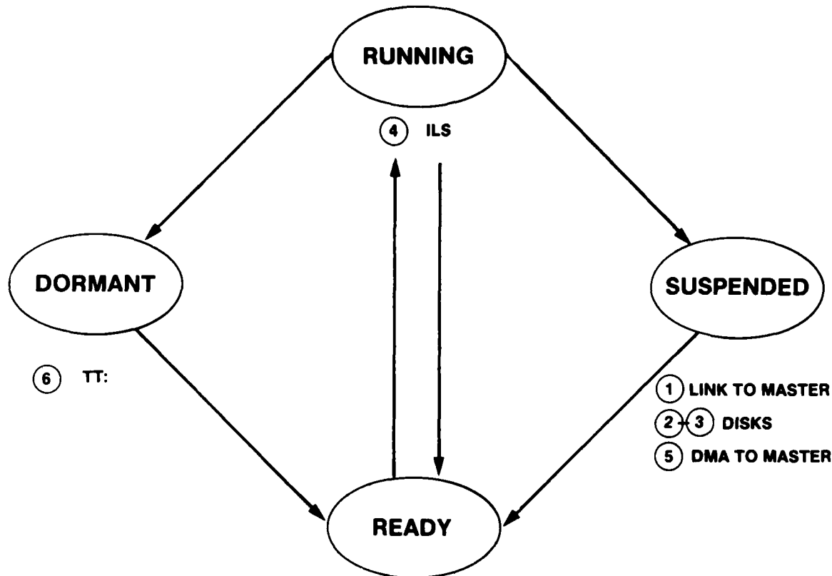
Figure 9 — Number Cruncher, A Functional View of the Software
