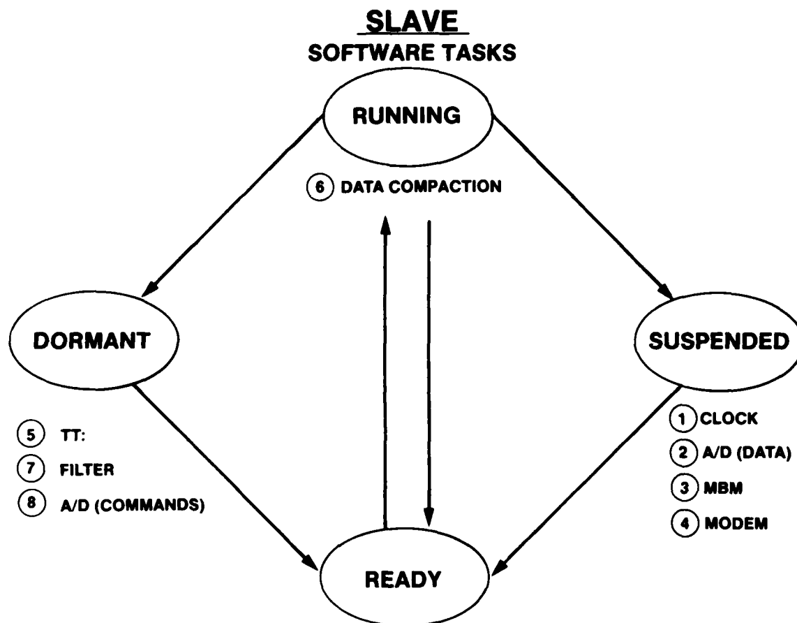
Figure 13 — Slave, A Functional View of the Software
