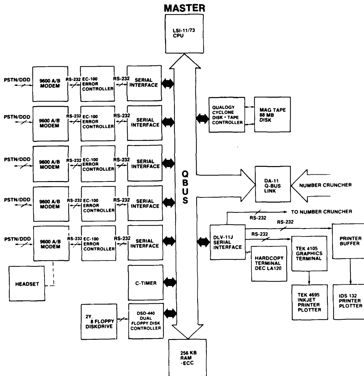
Figure 4 — Master, A Functional View of the Hardware
