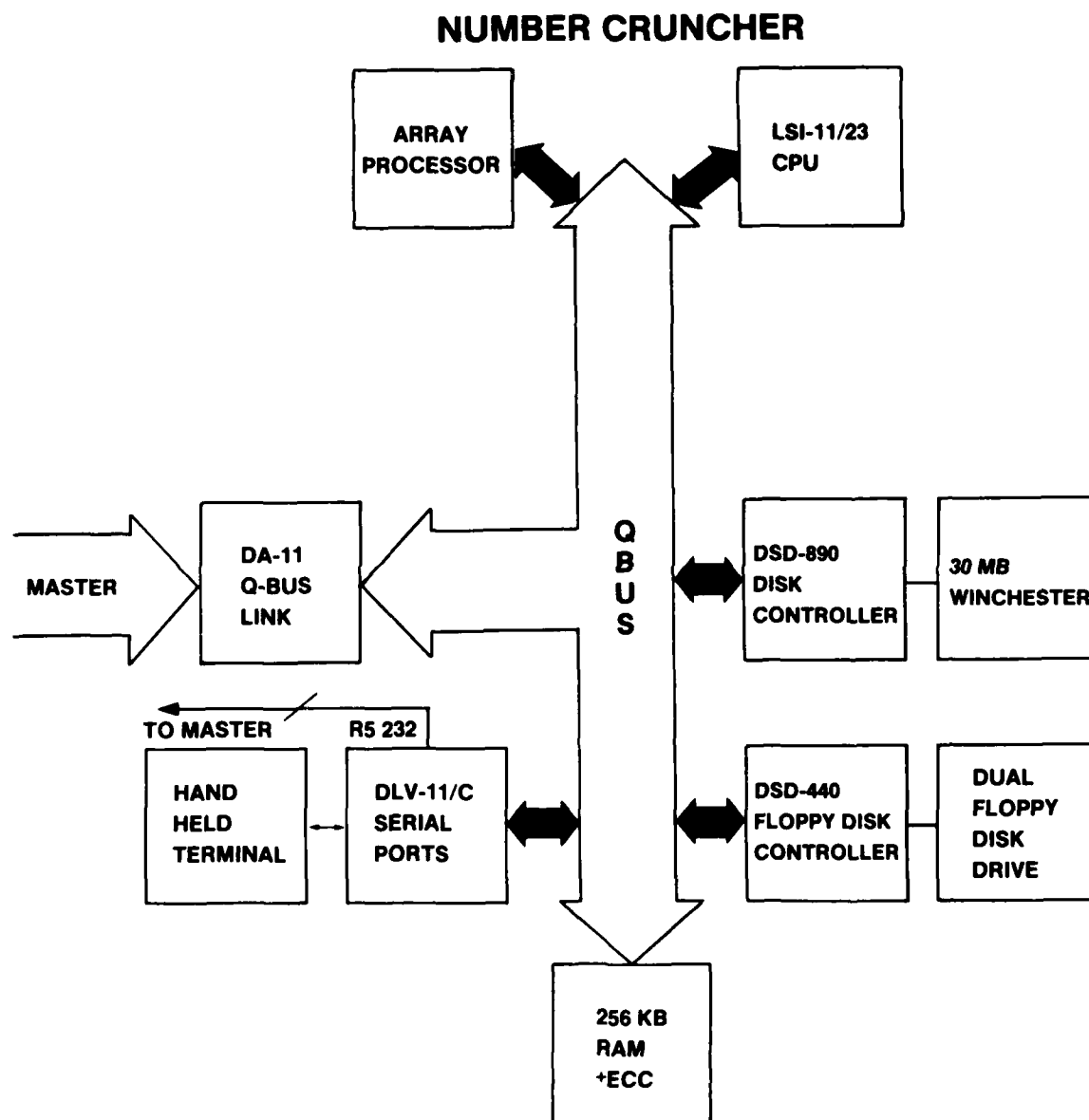
Figure 8 — Number Cruncher, A Functional View of the Hardware
