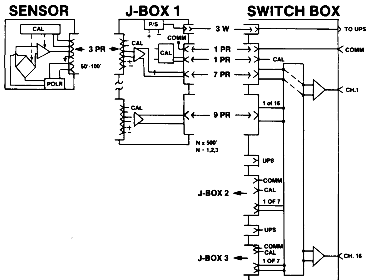
Figure 14 - The Sensor Tree
