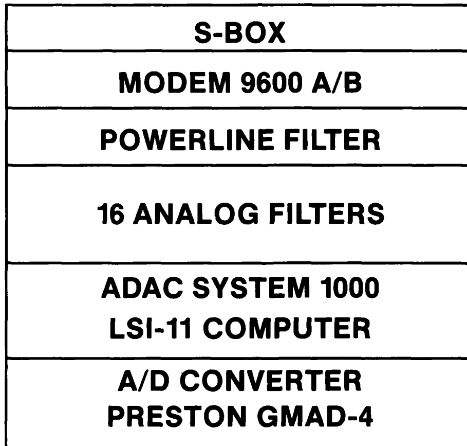
Figure 10 — Slave, Layout of Components
