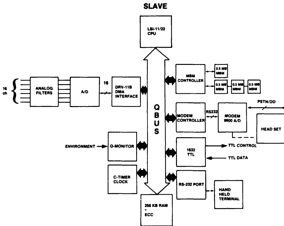
Figure 12 — Slave, A Functional View of the Hardware
