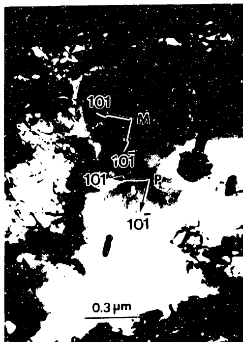
Fig. 1. Micrograph of grain oriented to a mixture of argon and 1% hydrogen. The approximate orientation relationship between the matrix (M) and the nucleated (P) is:
