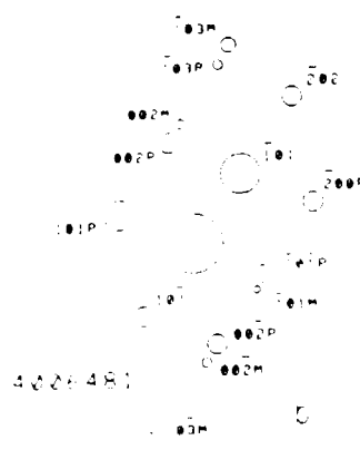
Fig. 2a and b: a: The micrograph of a grain oriented to a mixture of argon and 1% hydrogen. The approximate orientation relationship between the matrix (M) and the nucleated (P) is: b: Schematic diagram of the orientation of nucleated spots. Symbol M or P stands for the matrix or the nucleated spot, respectively.
