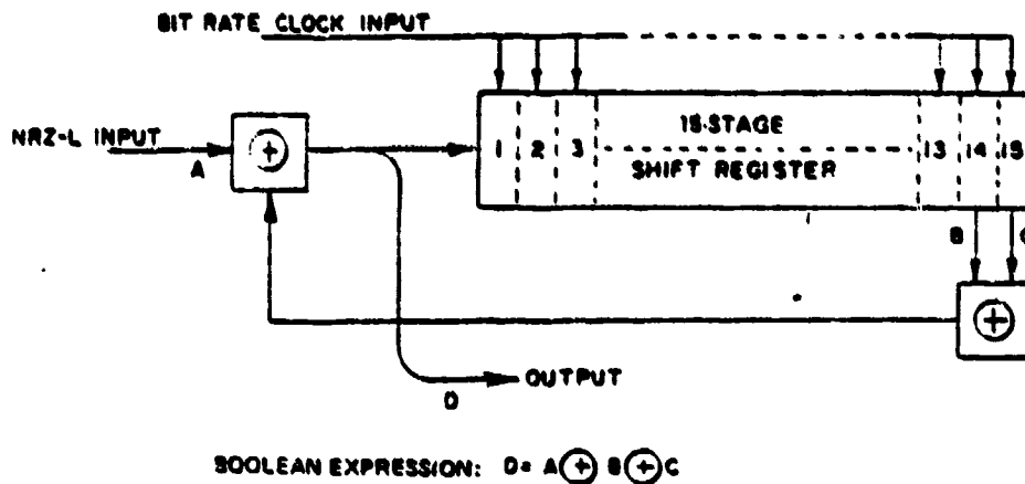
Figure 5.4-20. Randomizer.
