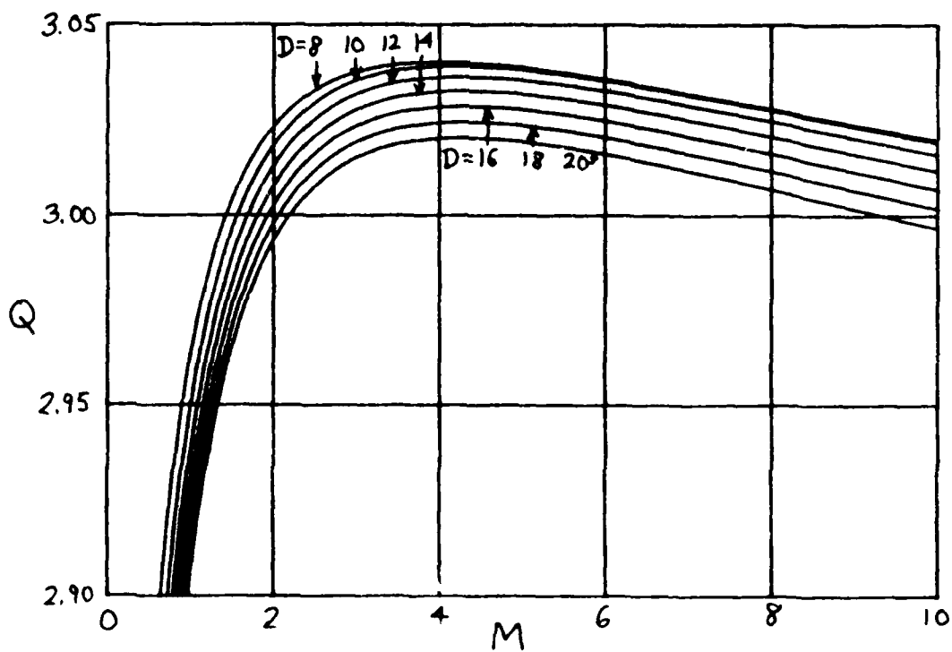
Figure H-7. Quality Ratio for \theta_0 = 1 , E_0/N_d = 20
