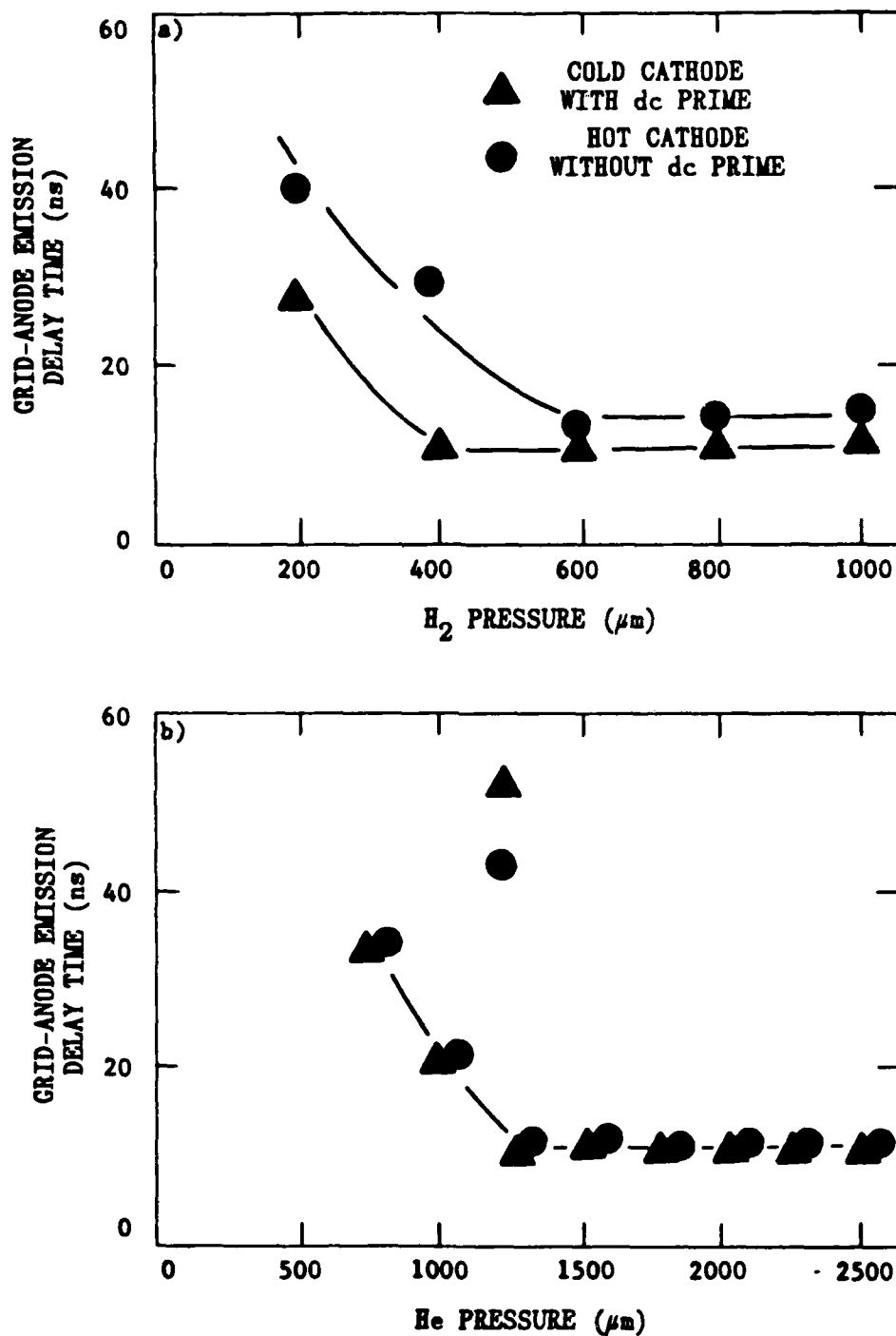
Figure 3-6. Time Delay for Plasma Emission from Opposite Ends of the Grid Anode Gap (a) Hydrogen, (b) Helium.
