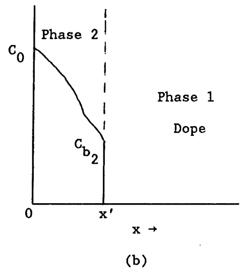
Figure 2.3. Moving boundary model for diffusion before and after formation of a second phase.
