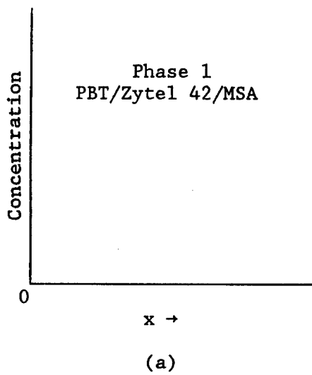
Figure 2.3. Moving boundary model for diffusion before and after formation of a second phase.
