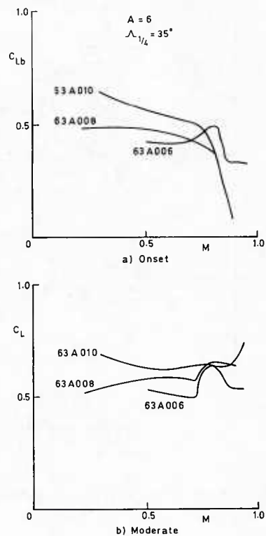
Fig 19 Effect of thickness/chord ratio on buffeting
