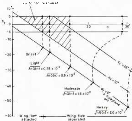
b) Wing flow and buffeting in first-bending mode
