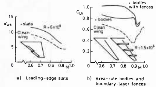
Fig 24 Alleviation of buffeting by wing modifications
