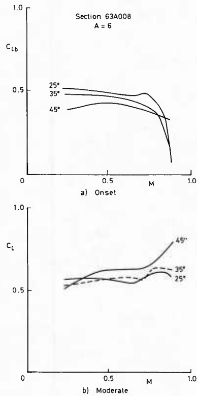
Fig 17 Effect of sweep ( \Lambda_1 ) on buffeting
