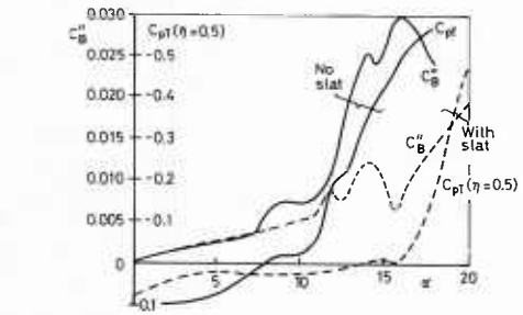
Fig 23 Example of the effect of leading-edge slats on buffeting (reference 35)
