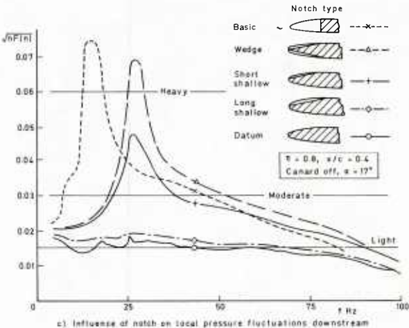
c) Influence of notch on local pressure fluctuations downstream
