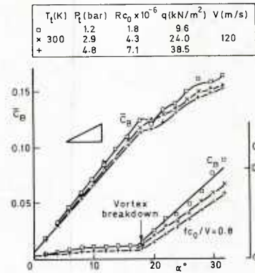
Fig 31 Influence of static aeroelastic distortion M = 0.35
