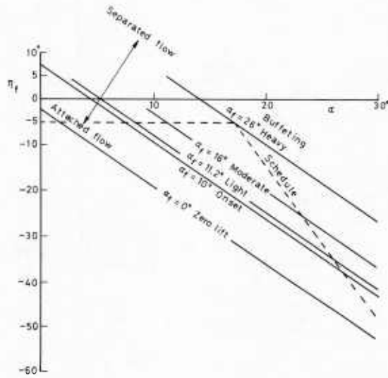
a) Foreplane flow and buffeting
