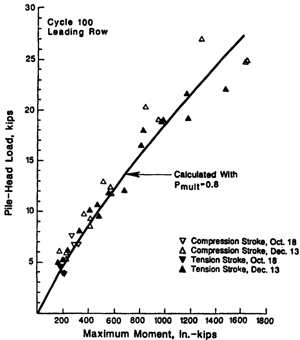
Fig. 7.12. Comparison of measured maximum moments for the cyclic case with the computed maximum moments for the leading row of piles.
