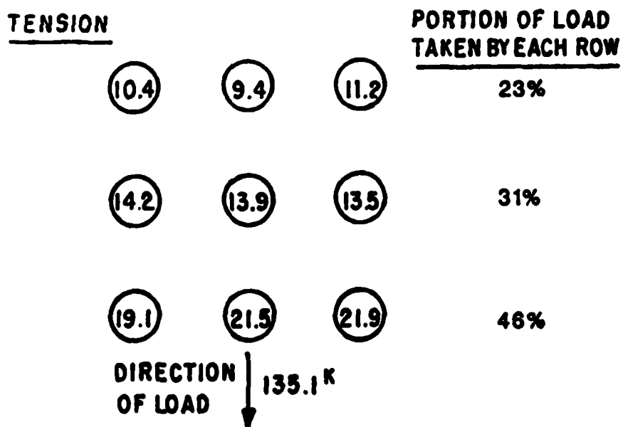
Fig. 5.27. Load distribution for load 5, cycle 100, pile-group test.
