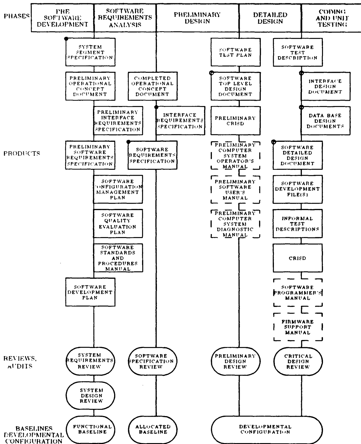
Figure 1-1: Software Development Cycle (per DOD-STD-2167)
