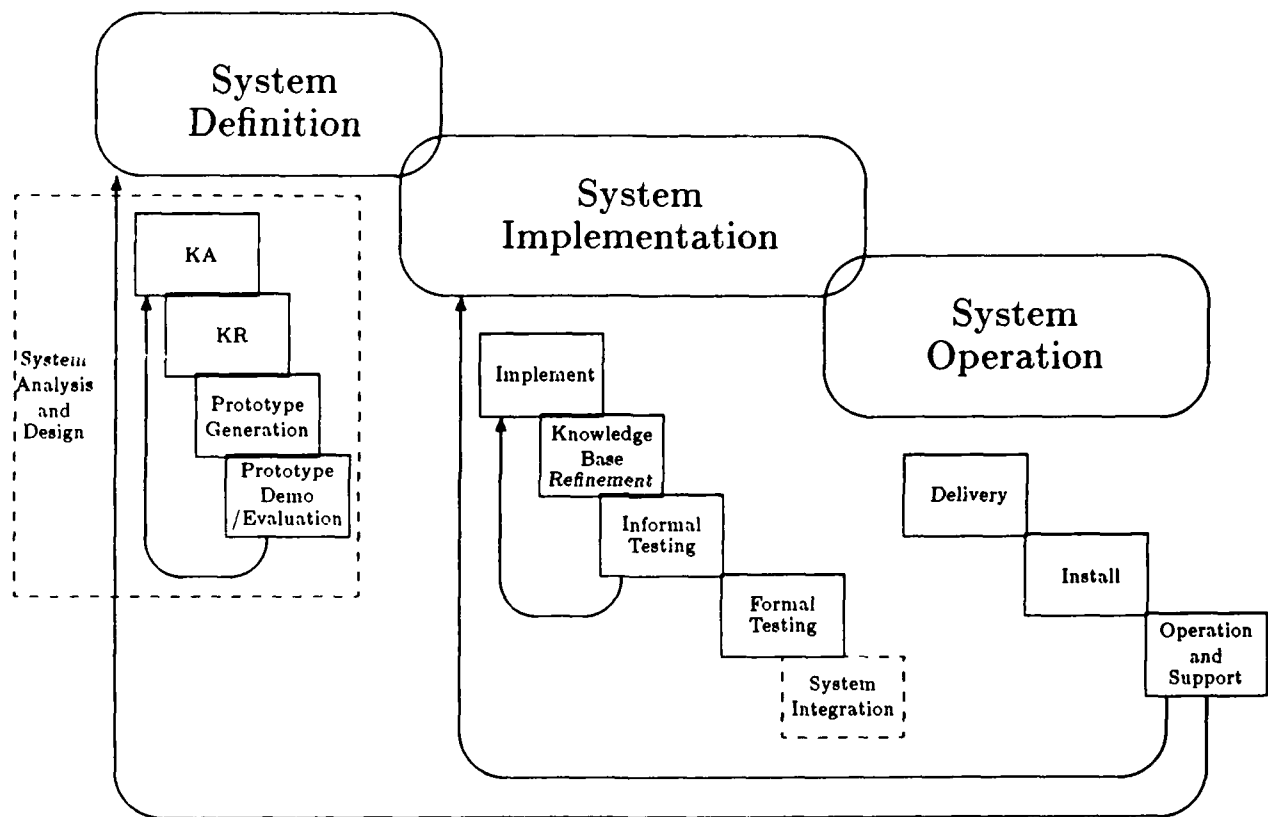
Figure 3-2: Detailed KBS Process Model
