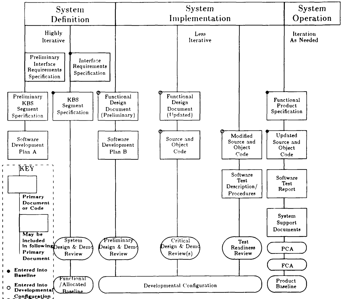
Figure 3-4: KBS Developer/Customer Interface Model
