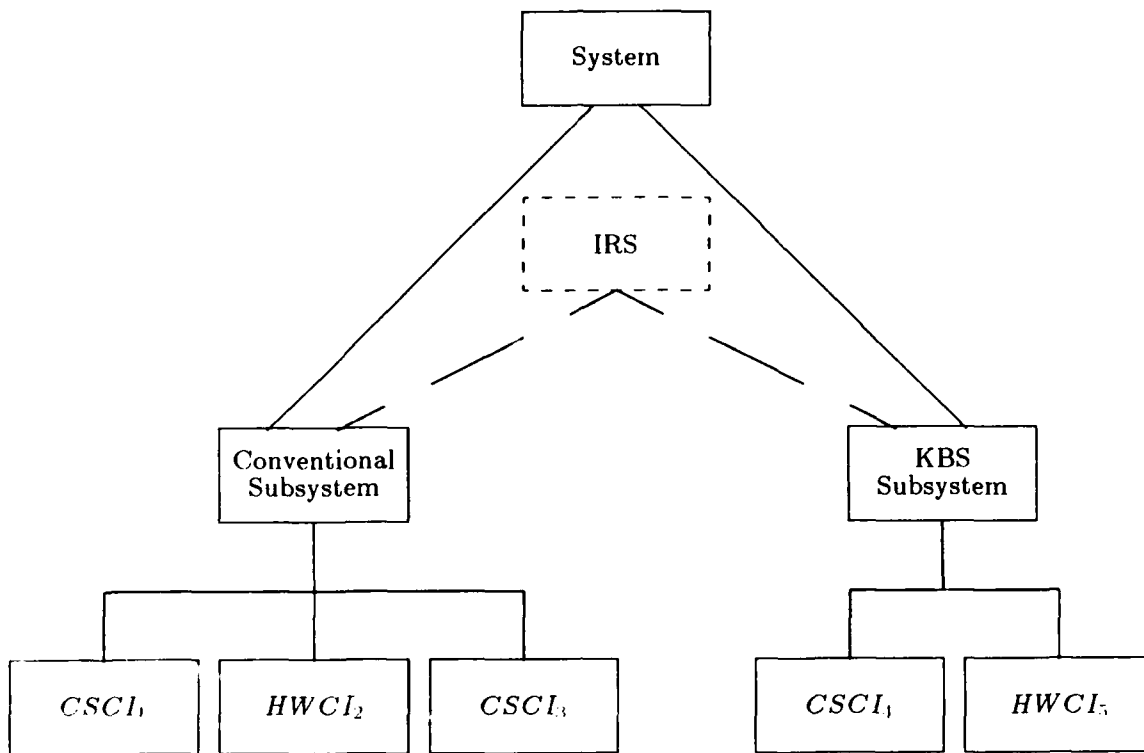
Figure 3-3: Sample Hybrid System Organization
