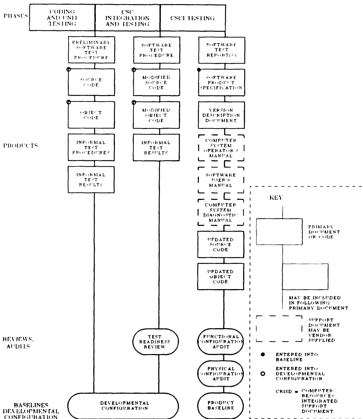
Figure 1-2: Software Development Cycle (Cont.) (per DOD-STD-2167)
