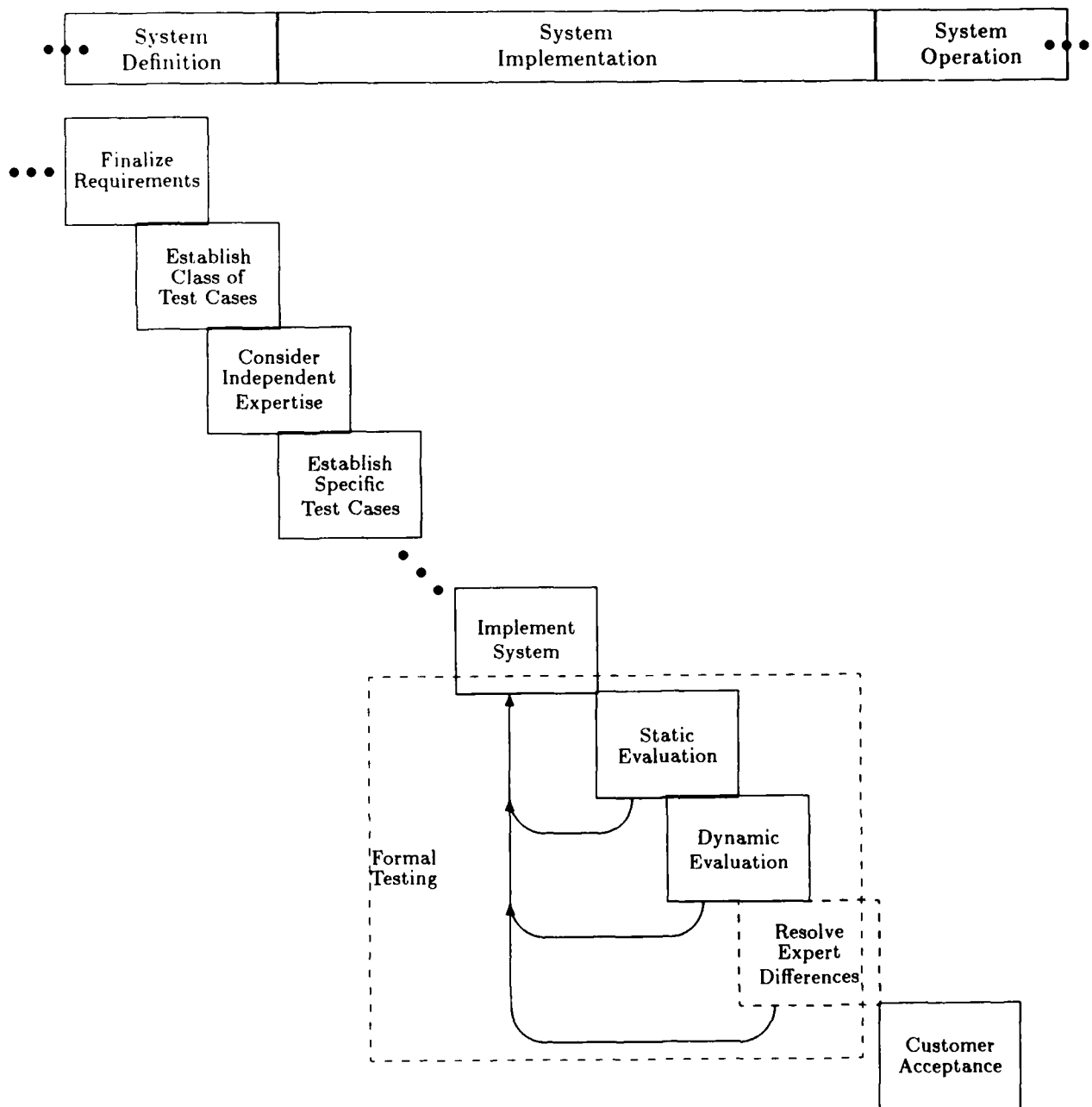
Figure 2-2: KBS Formal Test Approach
