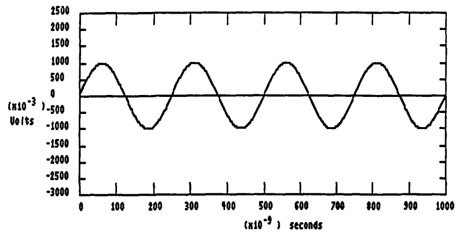
Figure 9. A 4-MHz sine wave in time domain after a forward and then inverse FFT.
