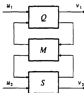
Figure 15.2 Associativity of Star Products
