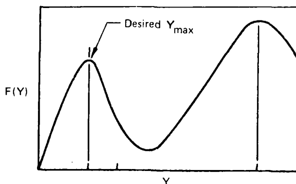
Figure 28. Behavior of Leeside Function F(Y) at High Angle-of-Attack
