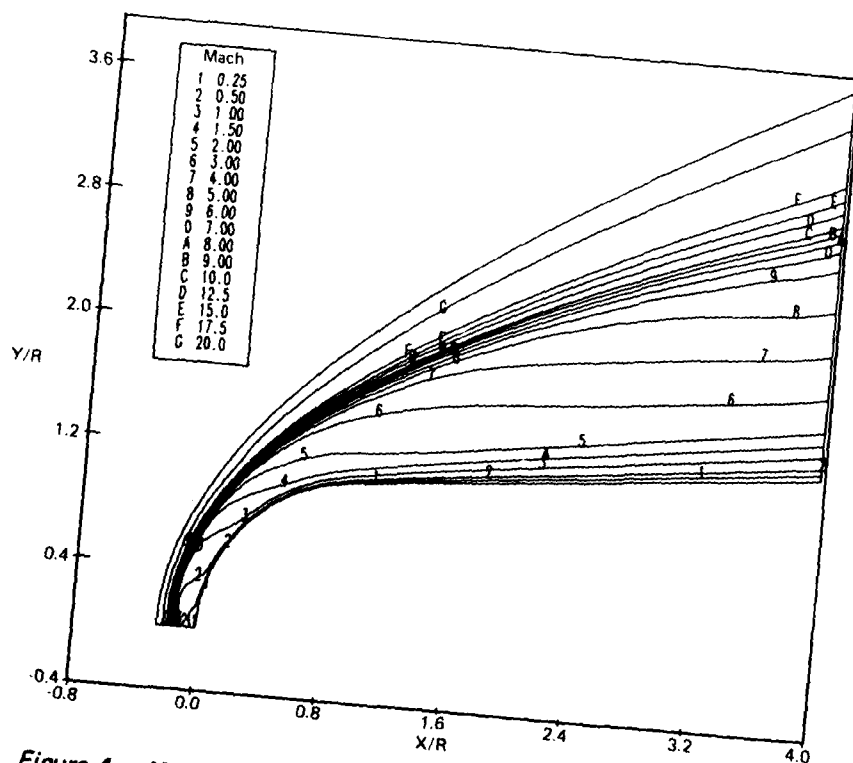
Figure 4a. Mach Contours for Three-Dimensional Blunt Nose Test Case
