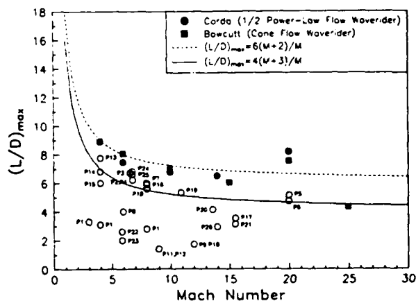
FIG. 1: Maximum lift-to-drag ratio comparison for various hypersonic configurations
