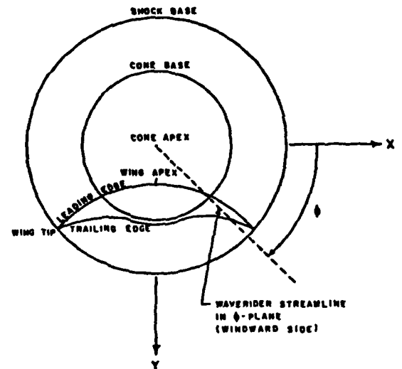
FIG. 7: Front view of a conical waverider with the generating cone and shock.
