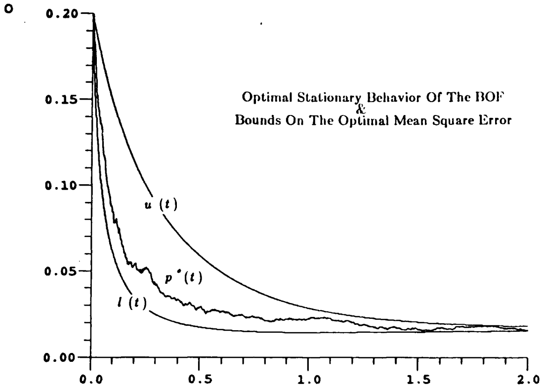
Figure 1: BOF performance
