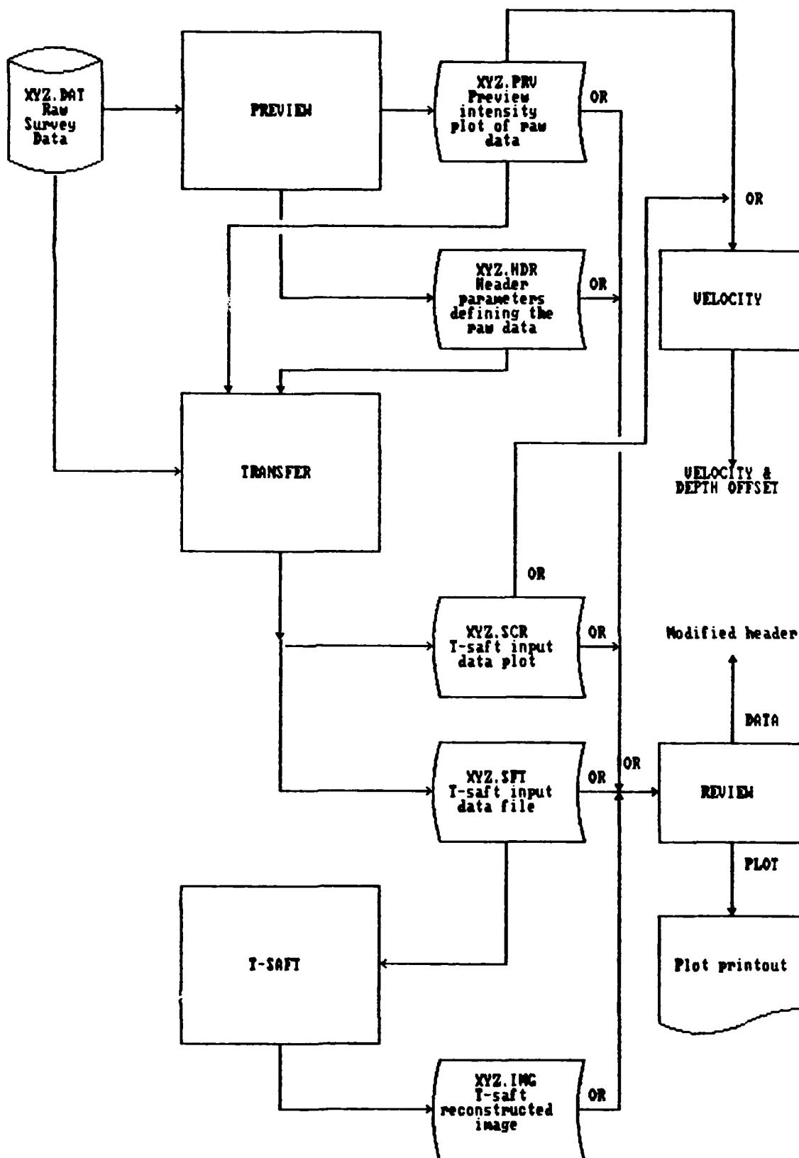
FIG 2-4 INPUT / OUTPUT FILES AND PROCESSING SOFTWARE RELATIONSHIP
