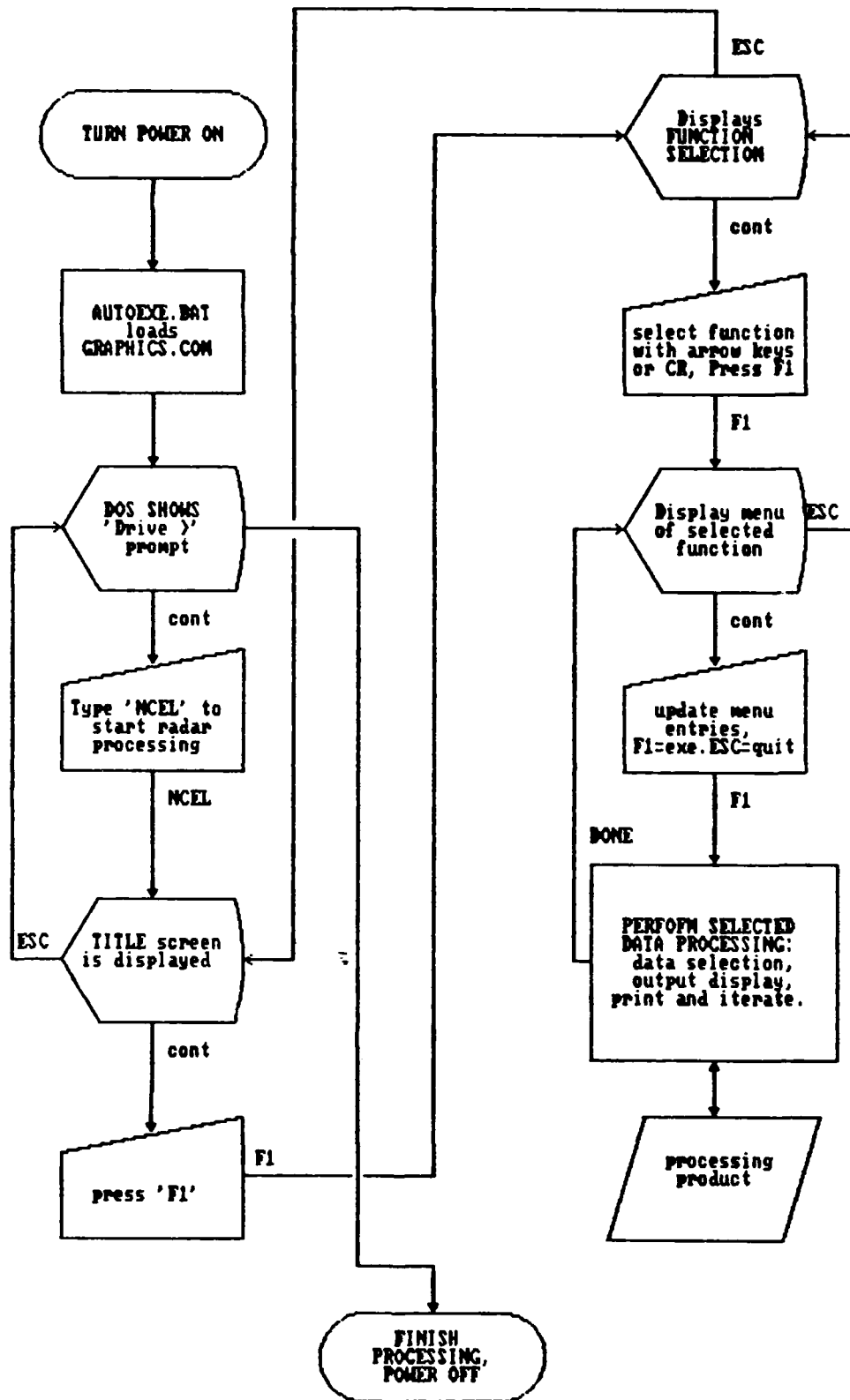
FIG 3-1 NCEL RADAR PROCESSING SOFTWARE PROGRAM EXECUTION FLOW
