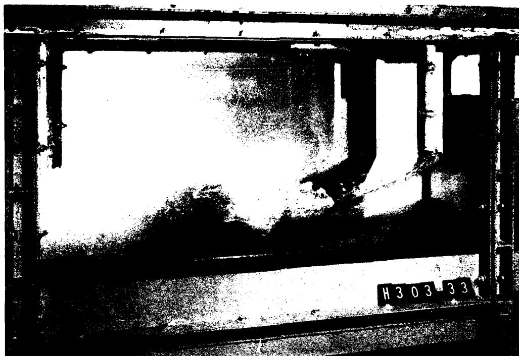
Photo 23. Hydraulic condition high bays = headwater el 50 ft, tail-water el 13 ft, gate opening 19.28 ft
