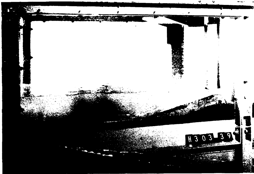
Photo 29. Hydraulic condition high bays = headwater el 20 ft, tail-water el 15 ft, gate opening 4.20 ft
