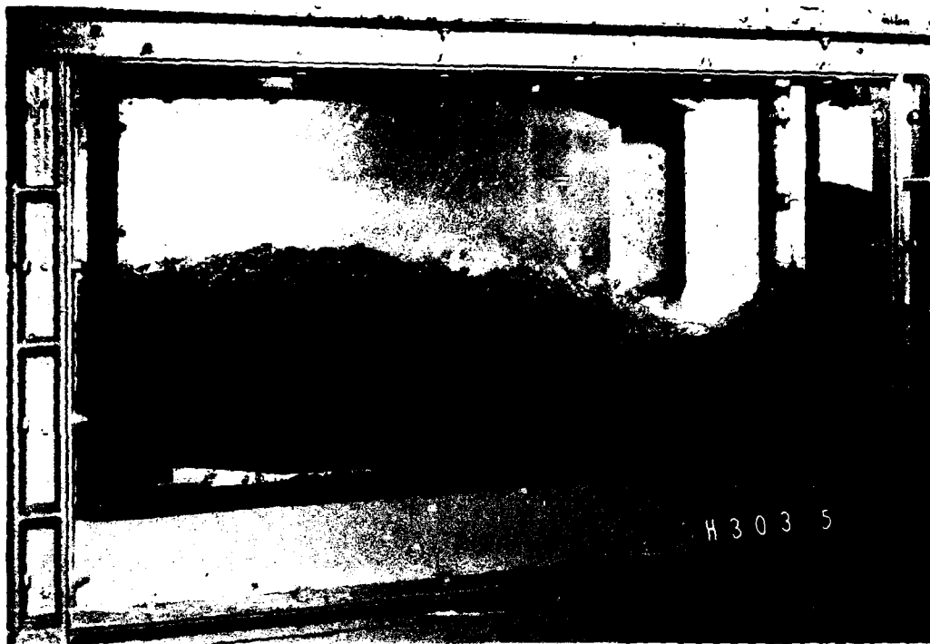
Photo 3. Hydraulic condition low bays = headwater el 40.0 ft, tailwater el 24.0 ft, gate opening 28.94 ft
