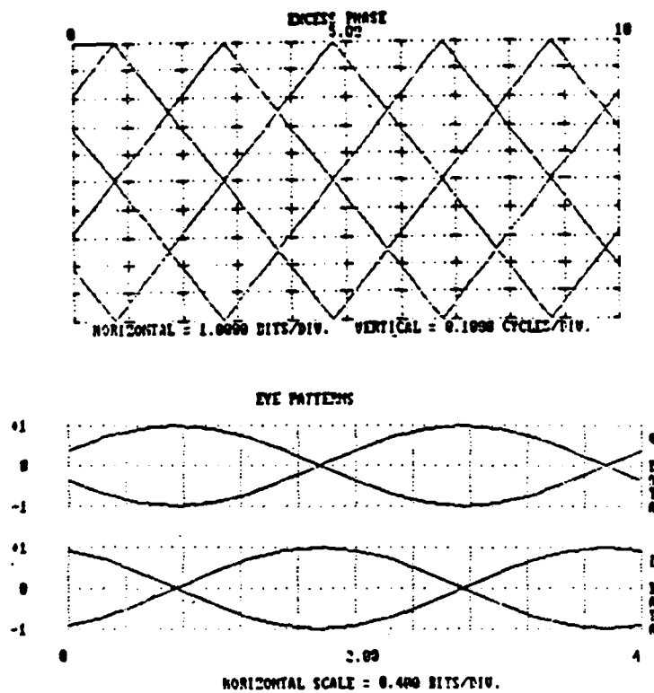
Figure 5.6 Phase Trellis and Eye Pattern for MSK.
