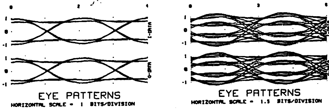
Figure 5.5 Eye Patterns for QPSK and 8PSK.
