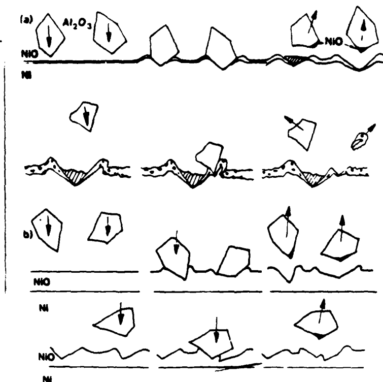
Figure 15. Steps in the erosion-oxidation mechanism of nickel. (a) clean nickel surface, \text{Al}_2\text{O}_3 particles embed and both metal and oxide deform plastically on impact until fracture. (b) Nickel with thick preoxidized scale, plastic deformation of oxide and cracking reduce thickness until conditions of (a) develop.
