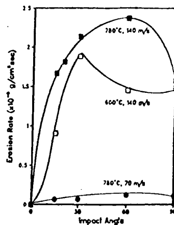
Figure 6b. Angular dependence of the erosion rate for the combined erosion and oxidation of cobalt at 780° and 600°C.
