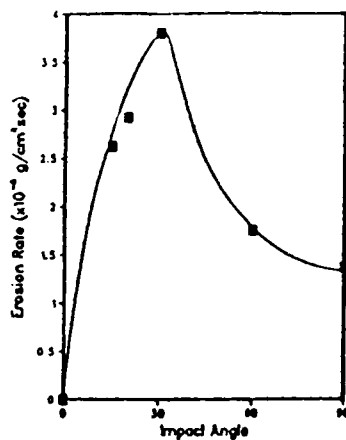
Figure 6a. Angular dependence of the erosion rate for the combined erosion and oxidation of nickel at 780°C and 140 m/s.
