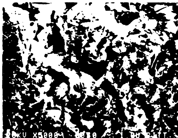
Fig. 7—NiO surface after erosion at 800^\circ\text{C} under 140 \text{ m/s}^{-1} airflow at 90 deg incidence for 50 min, showing evidence of plastic deformation and local melting.
