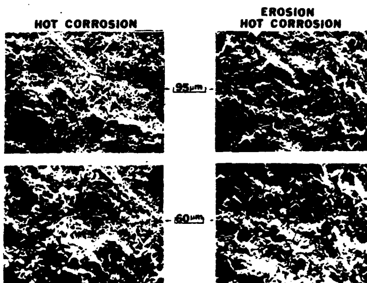
Figure 14. Scanning micrographs showing features of the oxide scales formed on IN738 after exposure to the hot corrosion test ( 0.05 \text{ mg/cm}^2 \text{ hr. Na}_2\text{SO}_4 -22% \text{K}_2\text{SO}_4 ) and the erosion-hot corrosion test ( 0.05 \text{ gm/cm}^2 \text{ hr. Na}_2\text{SO}_4 -22% \text{K}_2\text{SO}_4 , and 300 ppm 2.5 \mu\text{m } \alpha\text{-Al}_2\text{O}_3 particles) at 871^\circ\text{C} . The arrows identify the same areas at progressively higher magnifications. It is apparent that the erosive component has removed much of the porous oxide that is normally developed during hot corrosion attack.
