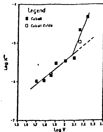
Figure 5. Summary of the relationship between the erosion rate constant and the particle velocity for the combined erosion and oxidation of cobalt and cobalt oxide at 780°C and 90° incidence.
