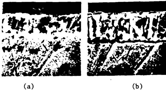
Figure 10 Comparison of oxide layers formed on cobalt after (a) erosion-oxidation at 800°C in 90 ms -1 airflow for 60 minutes and (b) oxidation only at 800°C in air for 60 minutes.
