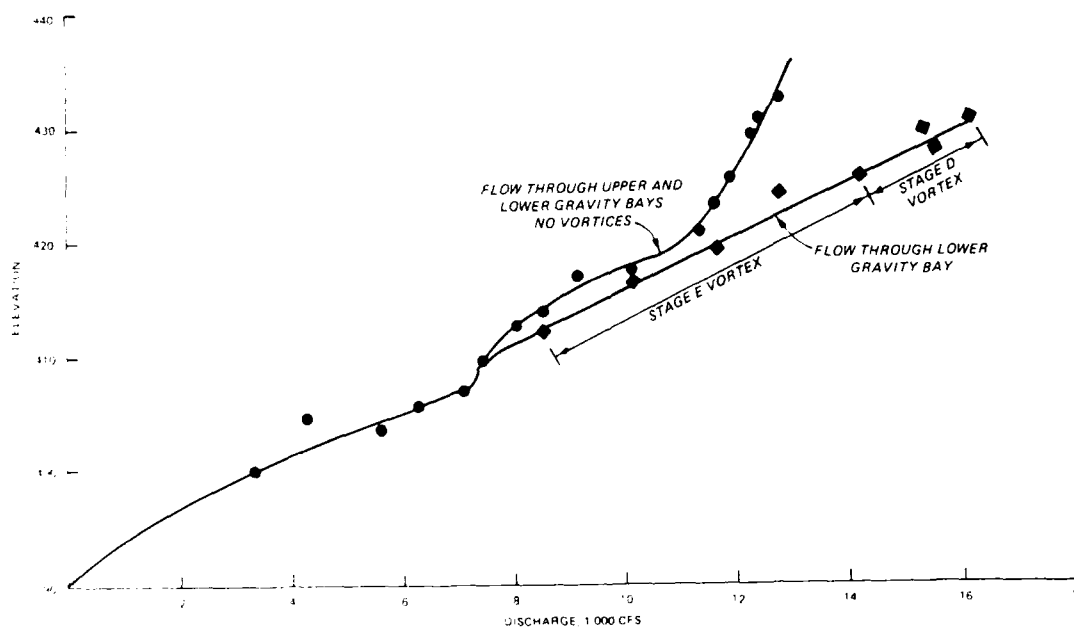
Figure 10. Rating curve, Scheme A type 3 gravity flow
