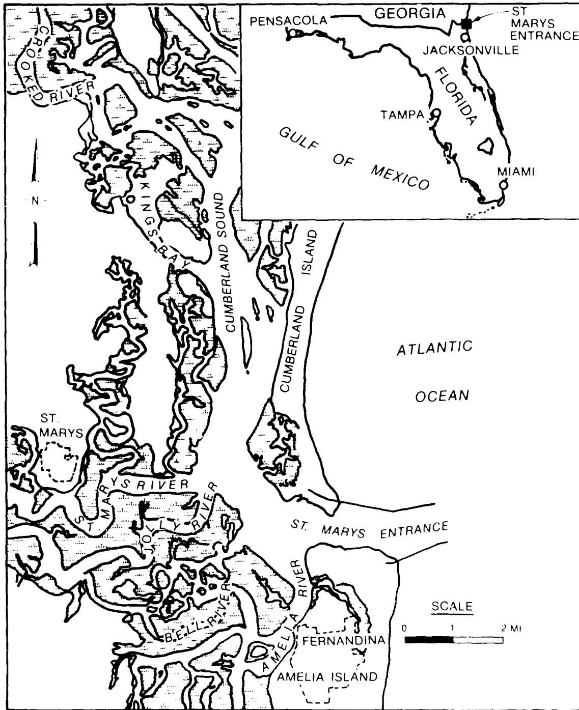
Figure 1. Location map
