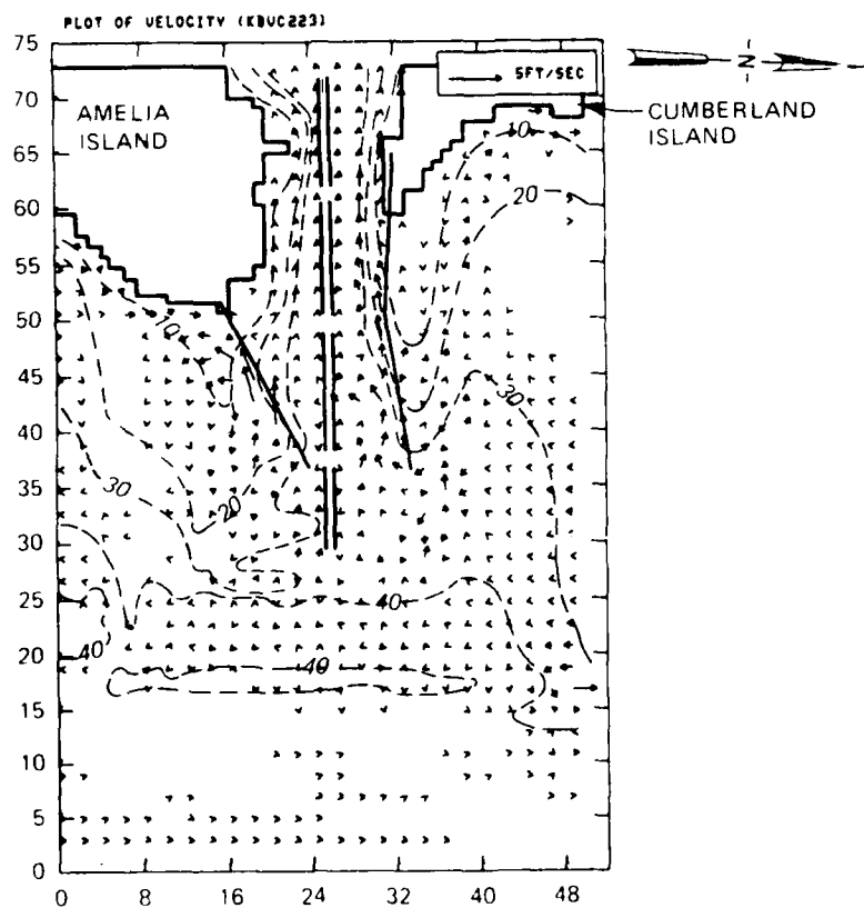
Figure 14. Wave-induced currents for Case A
