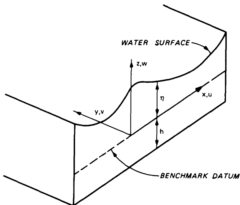
Figure 5. Coordinate system for WIFM
