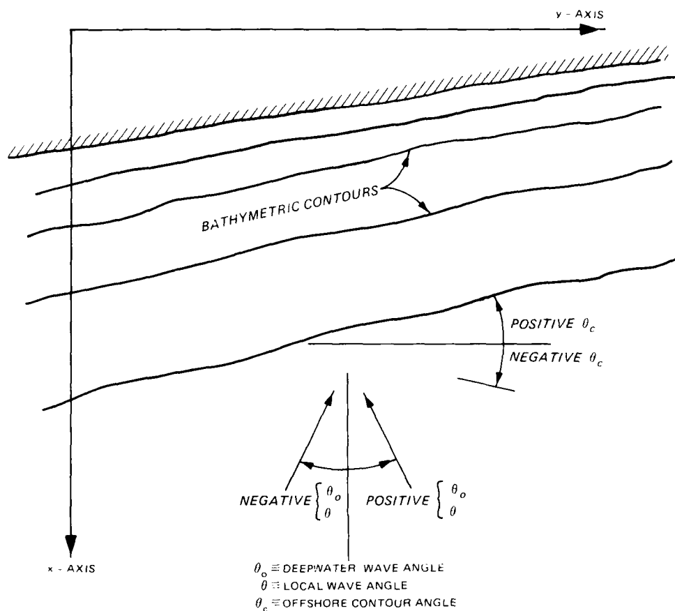
Figure 7. Definition of angle conventions used in RCPWAVE
