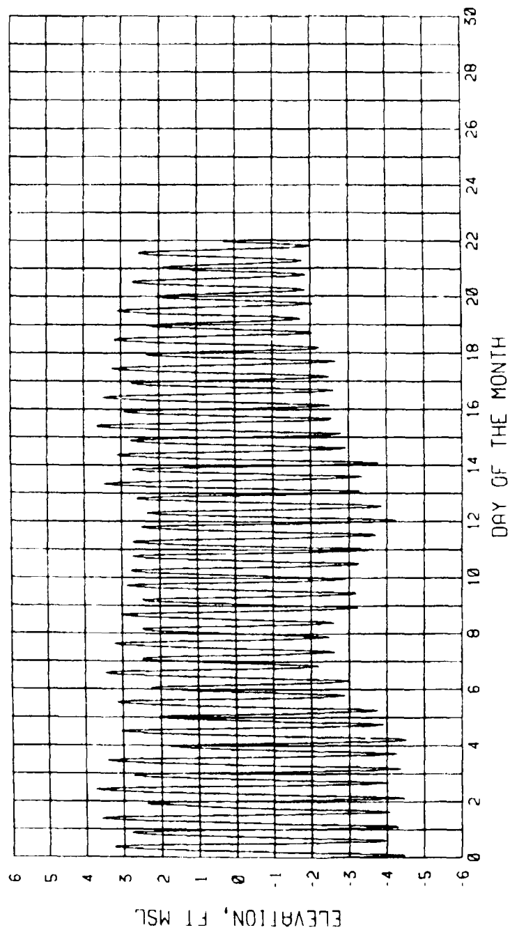
OBSERVED TIDAL ELEVATIONS NOVEMBER 1982 FERNANDINA BEACH, AMELIA RIVER
