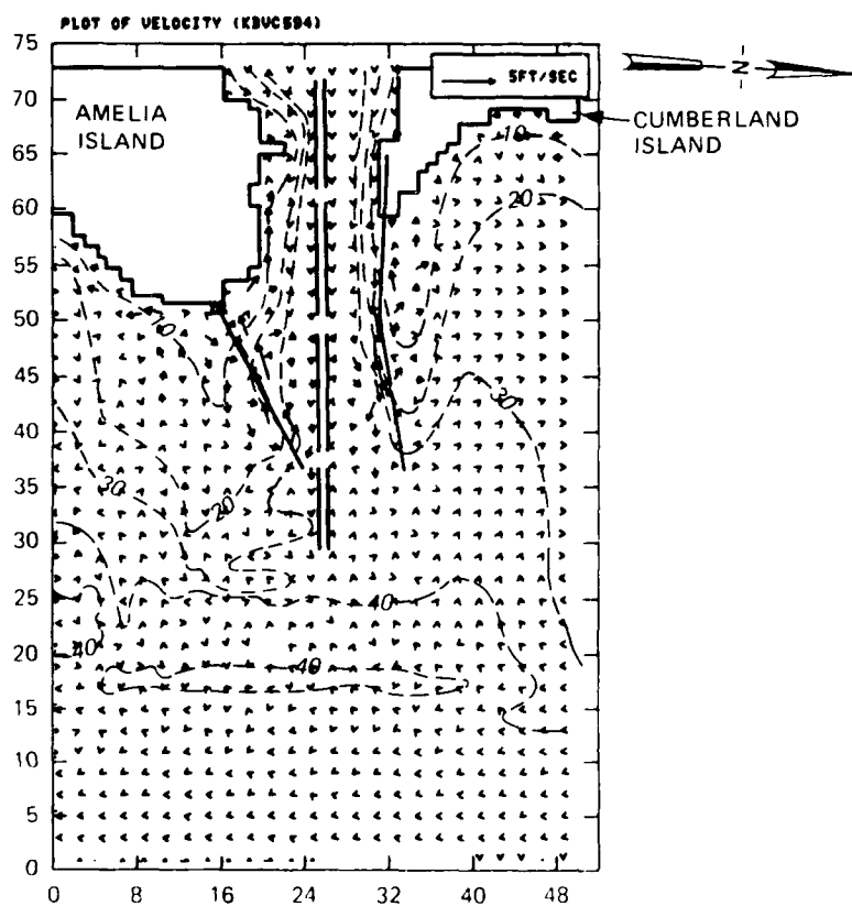
Figure 18. Wave-induced currents for Case C
