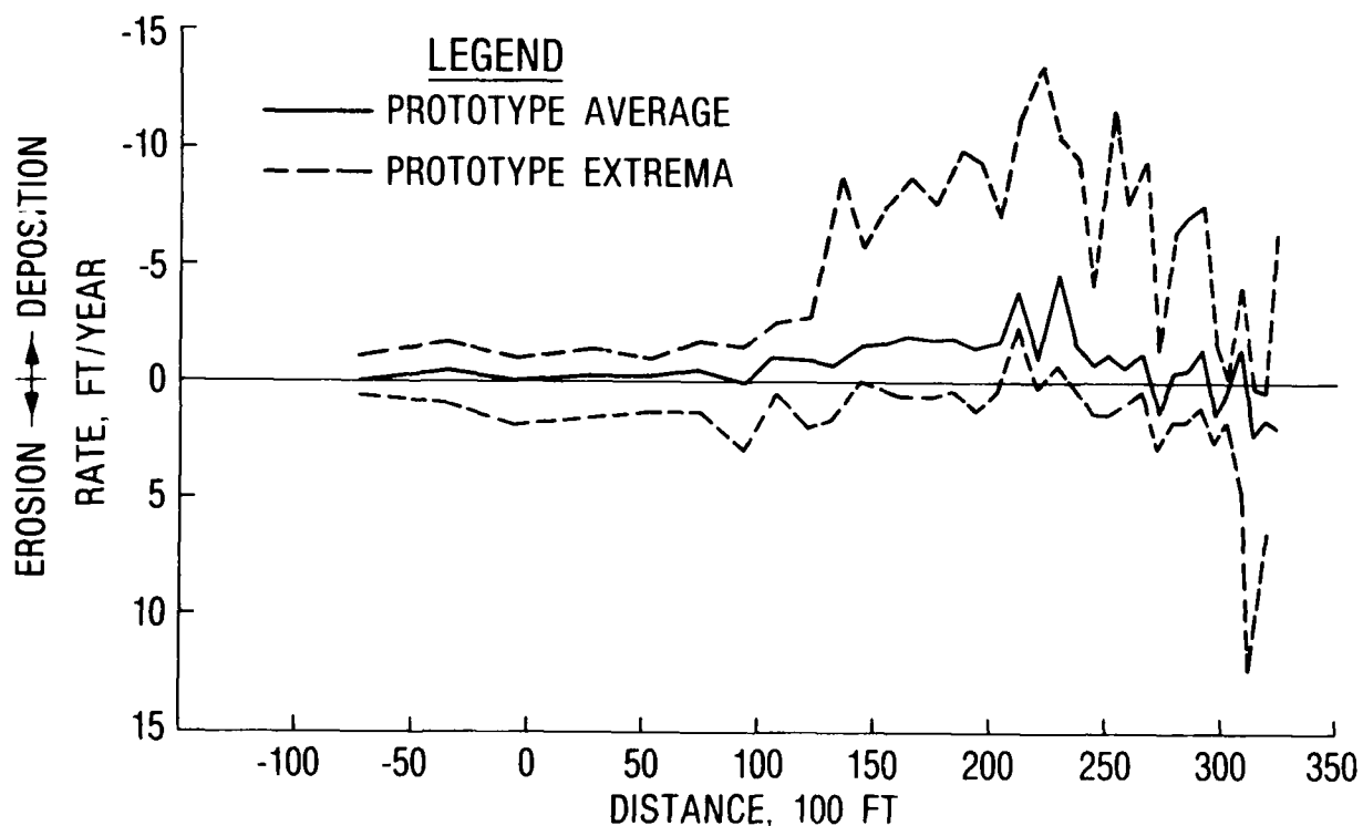
Figure 20. Prototype data on erosion/deposition rates
