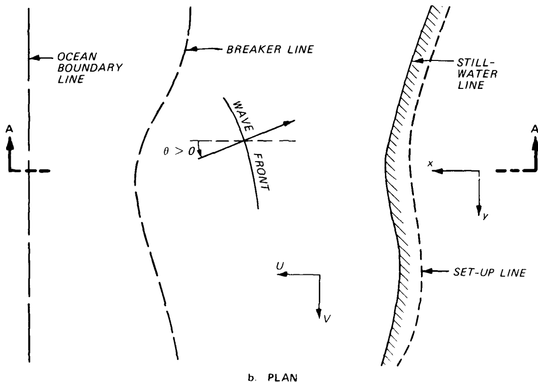
Figure 8. Definition sketch for an irregular beach (swl = still-water level)
