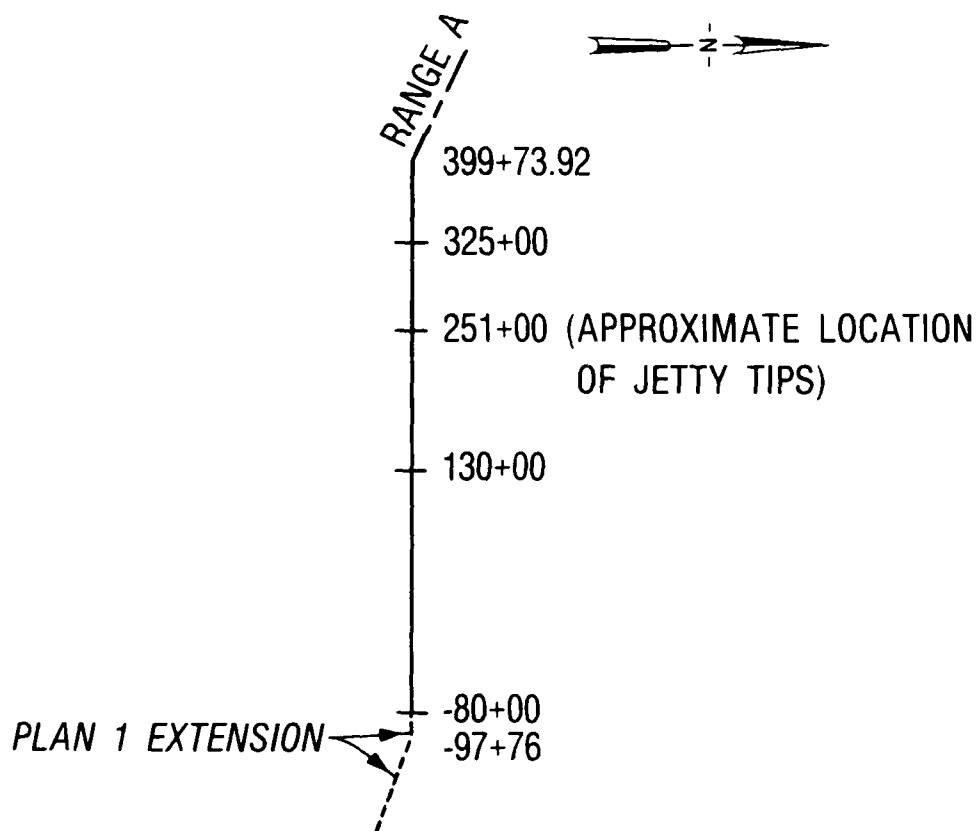
Figure 19. Pre-1985 CESAJ stationing
