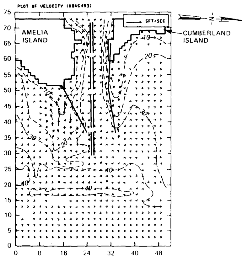
Figure 16. Wave-induced currents for Case B
