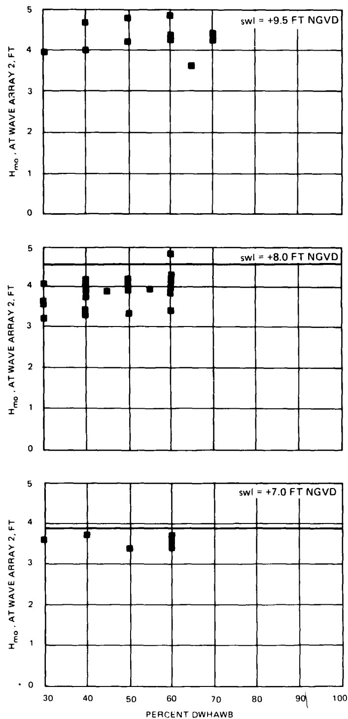
Figure 7. H_{mo} vs percent gain for Phase I seawall at swl's of +9.5, 8.0, and 7.0 ft NGVD (DWHAWB = design wave height at the wave board)
