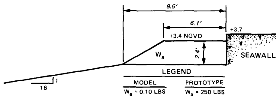
b. Exposed riprap toe as tested
