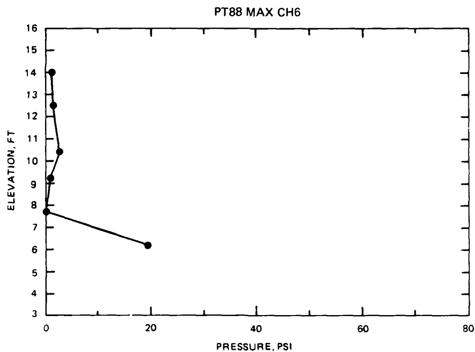
INSTANTANEOUS WAVE PRESSURE DISTRIBUTION HURRICANE PT88 SWL = +7.0 FT MAXIMUM PRESSURES ON CHANNELS 5 AND 6
