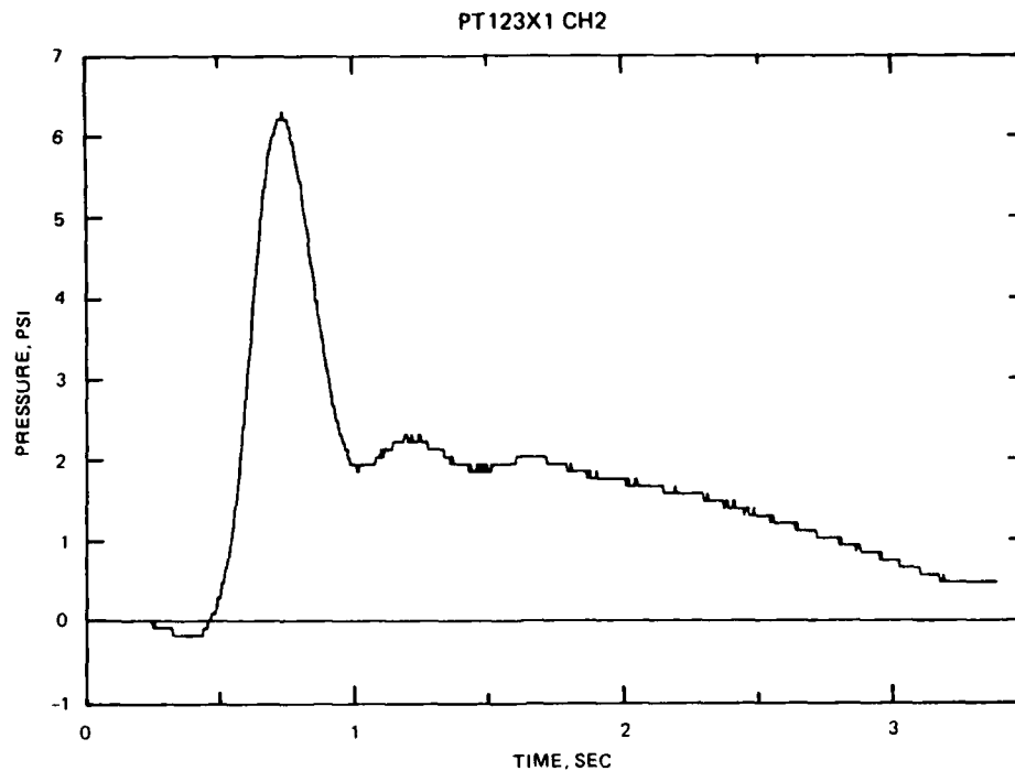
Figure 14. Typical maximum pressure record for Channel 2
