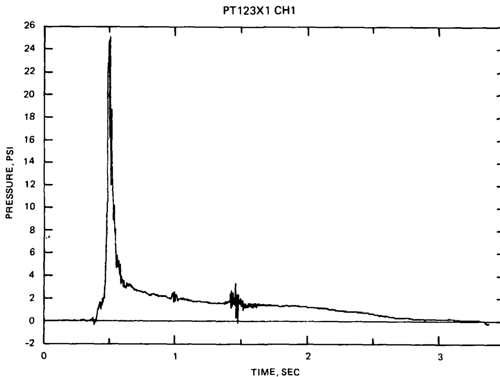
Figure 15. Time-history showing typical surge pressure
