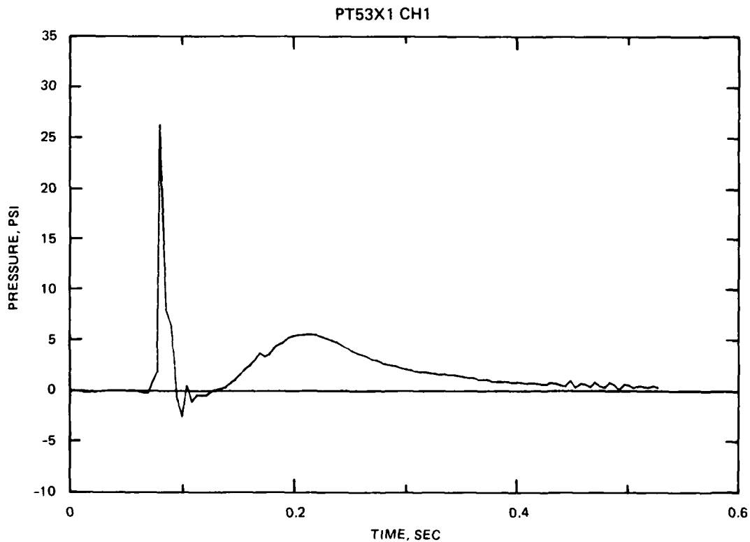
Figure 12. Typical wave pressure time-history
