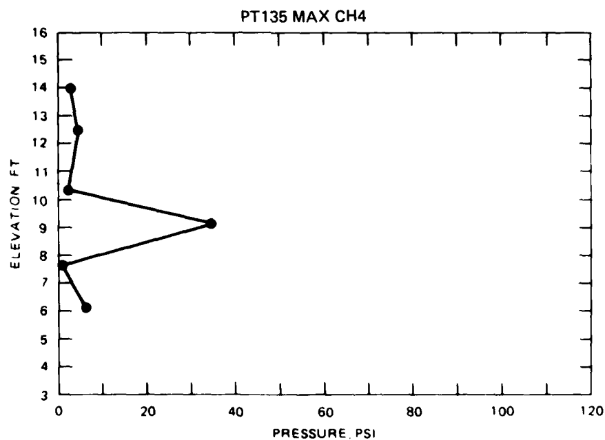
INSTANTANEOUS WAVE PRESSURE DISTRIBUTION HURRICANE PT135 SWL = +9.5 FT MAXIMUM PRESSURES ON CHANNELS 3 AND 4
