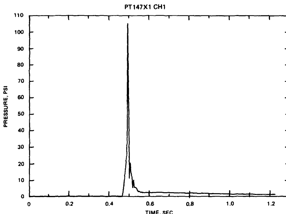
Figure 13. Time-history depicting typical shock pressure
