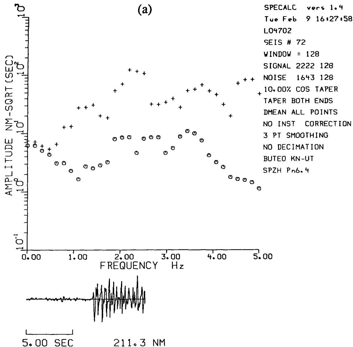
Figure 6. Vertical-component displacement amplitude spectra (symbol +), not corrected for instrument response, of Pn (based on 6.4 sec long window with 10% cosine taper) recorded at KN-UT for the seven explosions listed in Table III. Spectra of an equal window length of noise are also included (symbol o).
