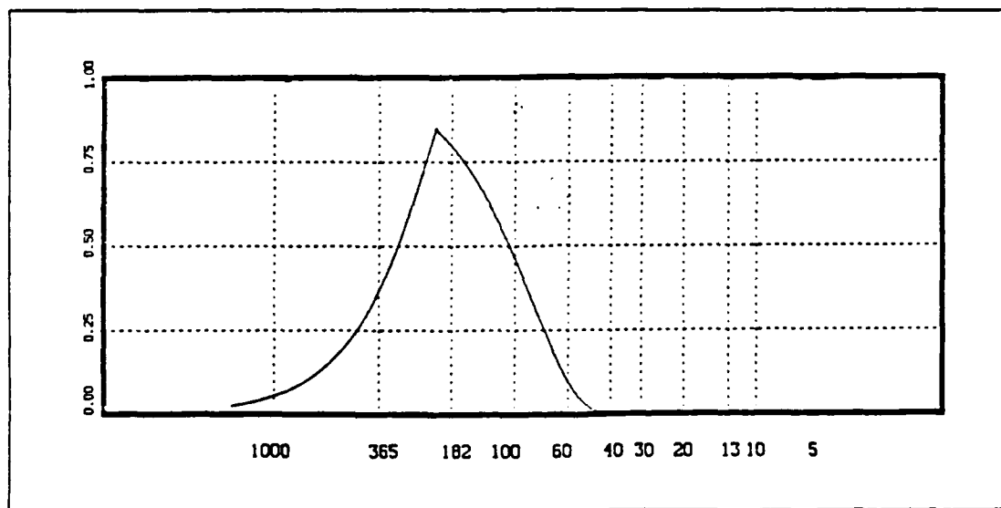
Fig. 20. Filter to isolate semiannual terms: Combination of twice run 75-point \sin^2 weighted filter and 183-point unweighted subtraction moving average. Maximum response is at about 200 days.
