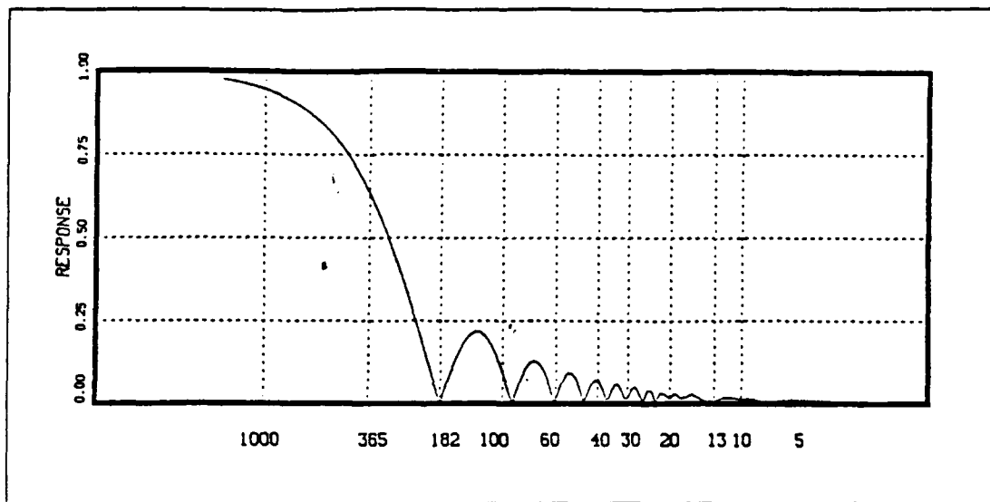
Fig. 19. Response of 183-point unweighted moving average filter: Used to isolate annual terms. A weighted filter would have required too many-points, and would not have sufficient vertical steepness to include annual frequencies. Still, almost 35% of the annual signal is attenuated in order to filter out the semiannual terms.
