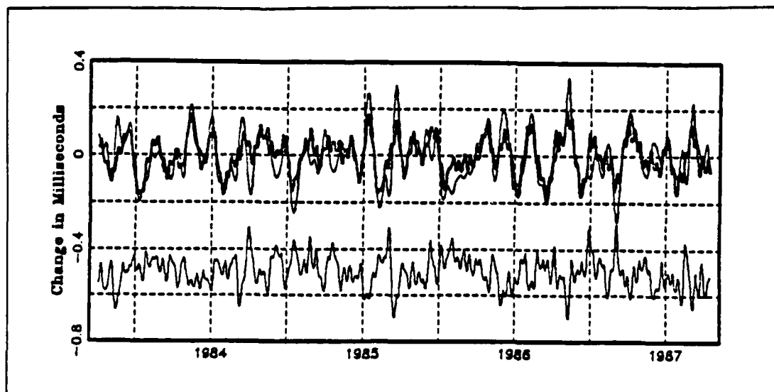
Fig. 7. Subseasonal Oscillations of \delta LOD_{atm} and \delta LOD_{USNO} : Residual of series depicted in Fig. 4 on page 23 subtracted from Fig. 3 on page 23. Bottom line is the difference of the two series shifted down 0.5 ms.
