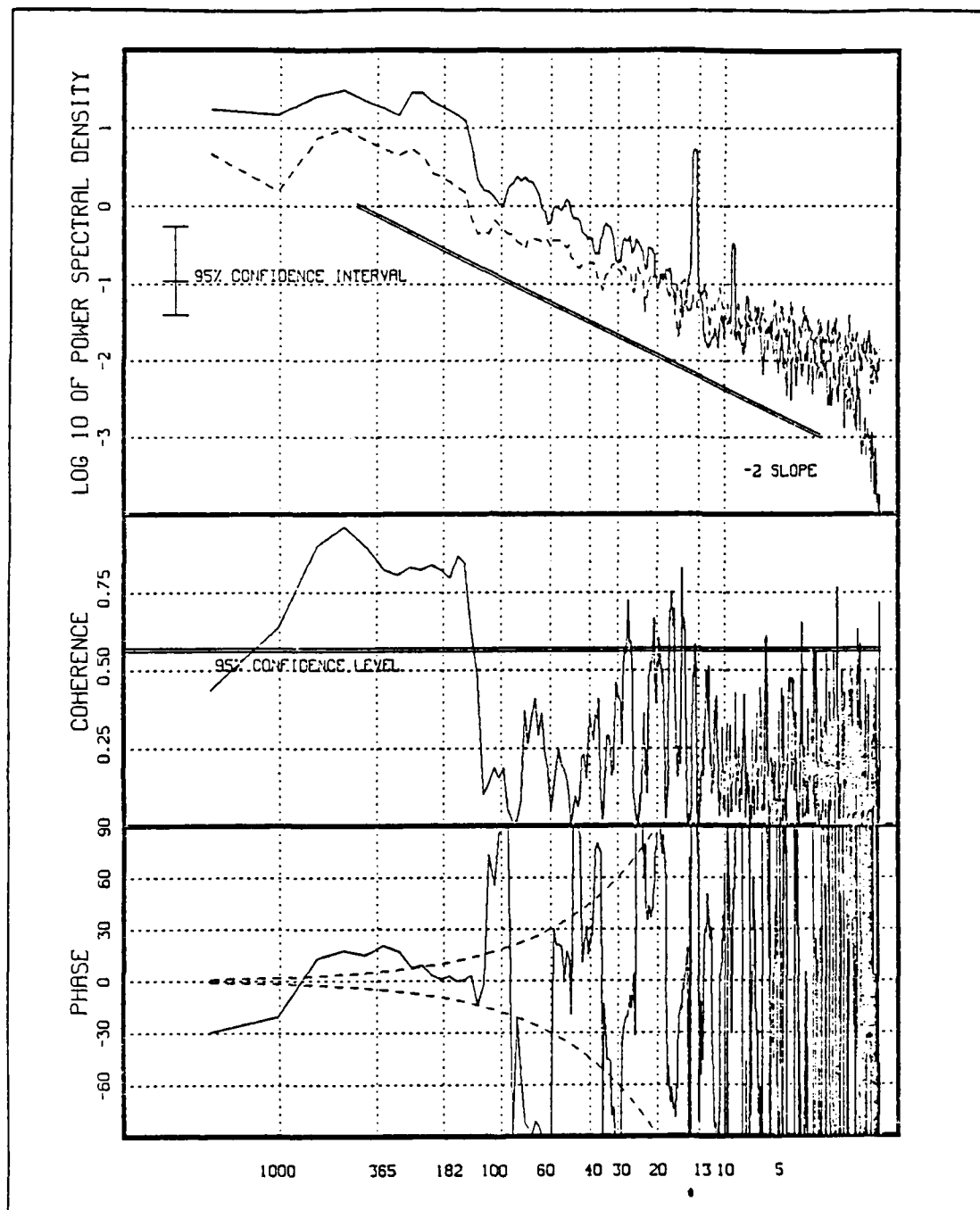
Fig. 16. Energy Density, Coherence, and Phase Spectra of \delta LOD_{USNO} and \delta LOD_{21m70^\circ} : As in Fig. 12 except the atmospheric signal is computed above 20^\circ N and below 20^\circ S .
