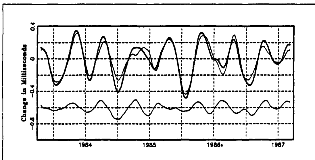
Fig. 6. Semiannual terms of \delta LOD_{USNO} and \delta LOD_{atm} : Heavy line is \delta LOD_{USNO} Bottom graph is residual of \delta LOD_{USNO} - \delta LOD_{atm} shifted down by 0.5 ms. Frequency response of filter is Fig. 20 on page 48 of Appendix C.
