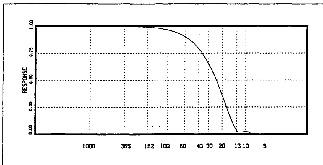
Fig. 17. Spectral response of 23-point \sin^2 weighted filter: Lowpass filter designed primarily to remove solid body tides at 7 and 13.5 days from \delta LOD_{USNO} data.
