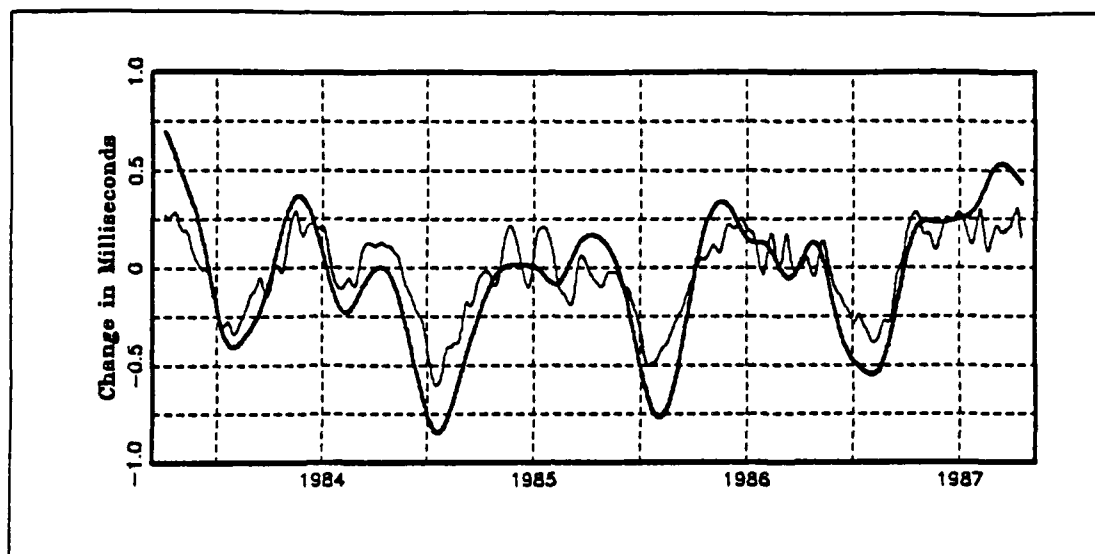
Fig. 11. Comparison of \delta LOD_{USNO\text{-}seasonal} and \delta LOD_{atm70} : Heavy line is USNO seasonal signal (from Fig. 6); light line is atmospheric signal derived from midlatitude components of atmospheric LOD above 20^{\circ}N and below 20^{\circ}S .
