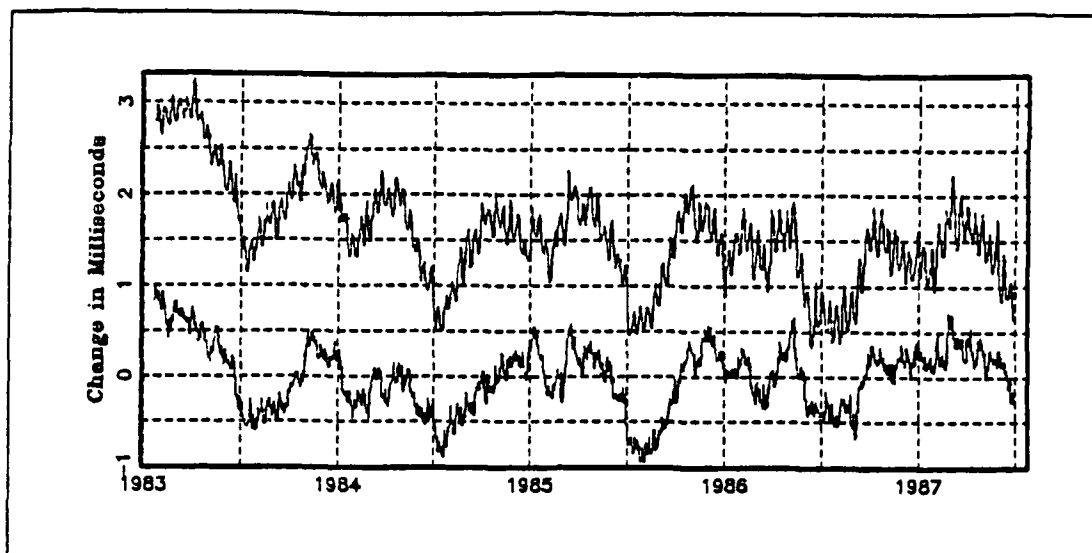
Fig. 1. Unfiltered time series of \delta LOD_{USNO} (top) and \delta LOD_{atm} (bottom): Note the linear, decreasing trend in the \delta LOD_{USNO} plot. The mean has not been removed from the USNO data.
