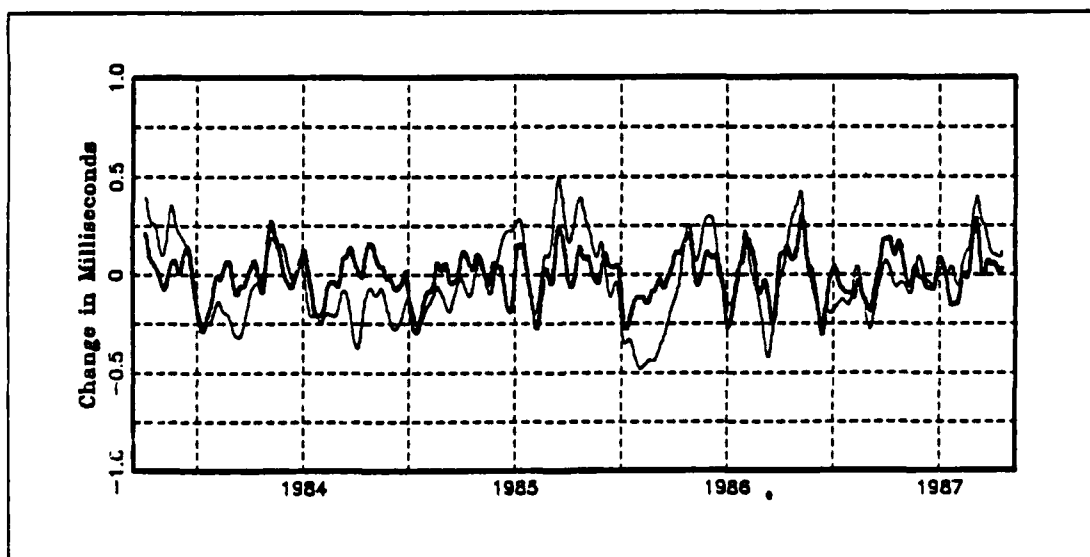
Fig. 8. Comparison of \delta LOD_{USNO-seasonal} and \delta LOD_{atm15} : Heavy line is \delta LOD_{USNO} seasonal signal; light line is \delta LOD_{atm15} derived from integrating atmospheric angular momentum within 15^\circ of the equator.
