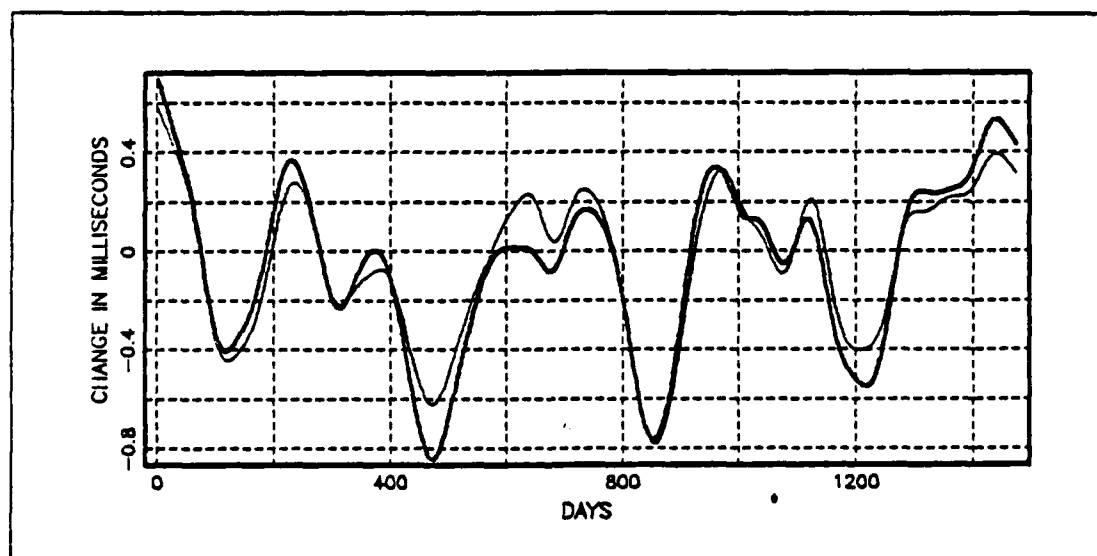
Fig. 4. Seasonal terms of \delta LOD_m and \delta LOD_{USNO} : Heavy line is USNO series. A 75-point weighted moving average filter was applied twice to each series; 148 points were lost from the ends.
