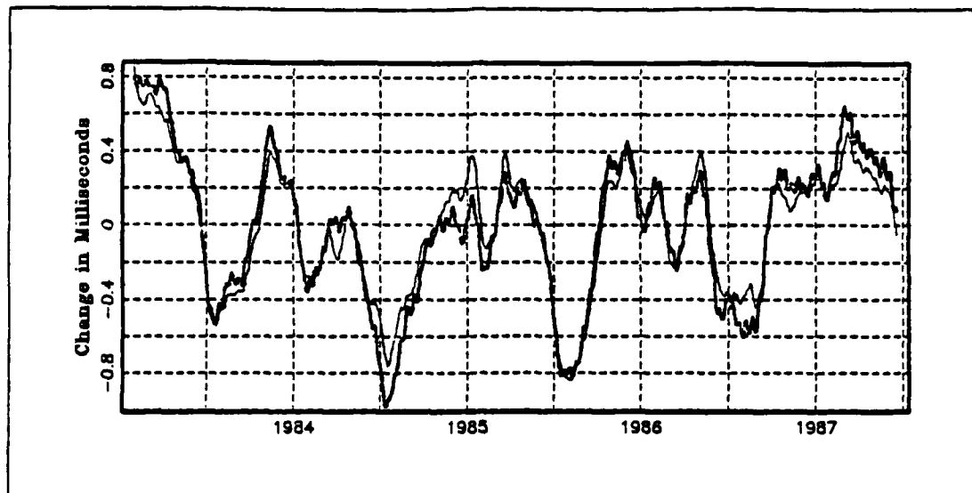
Fig. 3. Smoothed \delta LOD_m and \delta LOD_{USNO} series: A 23-point moving average filter was used to eliminate noise and high frequency tidal oscillations. Heavy line is the \delta LOD_{USNO} series.
