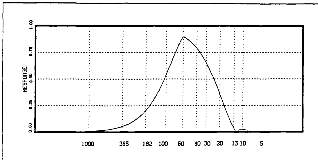
Fig. 21. Subseasonal isolation filter: Combination of twice run 75-point weighted moving average (see Fig. 19) and 23-point weighted moving average. Peak response is at 60 days.
