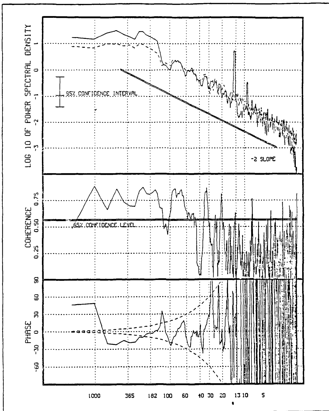
Fig. 15. Energy Density, Coherence, and Phase Spectra of \delta LOD_{USNO} and \delta LOD_{20^\circ} : As in Fig. 12 except the atmospheric signal is computed within 20^\circ of the equator.
