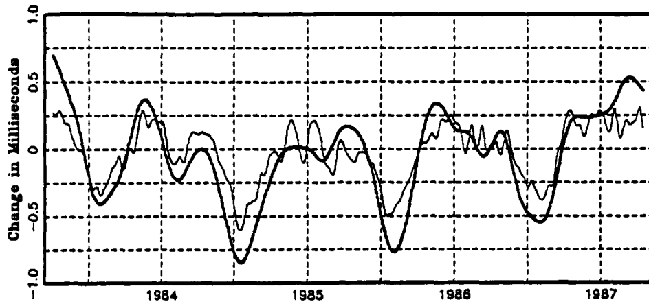
Fig. 9. Comparison of \delta LOD_{USNO-seasonal} and \delta LOD_{alm75} : Same as Fig. 8, except midlatitude components poleward of 15^\circ N and 15^\circ S are compared with seasonal terms of \delta LOD_{USNO} .
