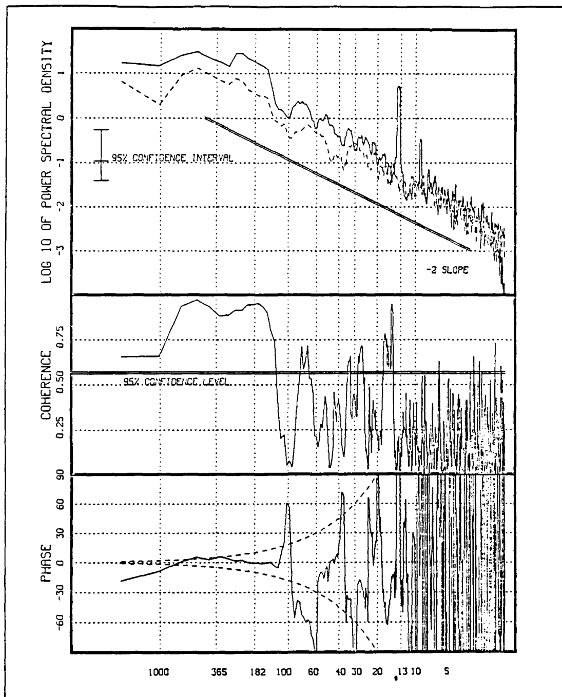
Fig. 14. Energy Density, Coherence, and Phase Spectra of \delta LOD_{USNO} and \delta LOD_n : As in Fig. 12 except the atmospheric signal is computed above 15^\circ N and below 15^\circ S .
