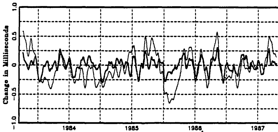
Fig. 10. Comparison of \delta LOD_{USNO-subseasonal} and \delta LOD_{alm20} : Heavy line is USNO sub-seasonal signal (from Fig. 7); light line is derived from integrating atmospheric angular momentum within 20^\circ of the equator.
