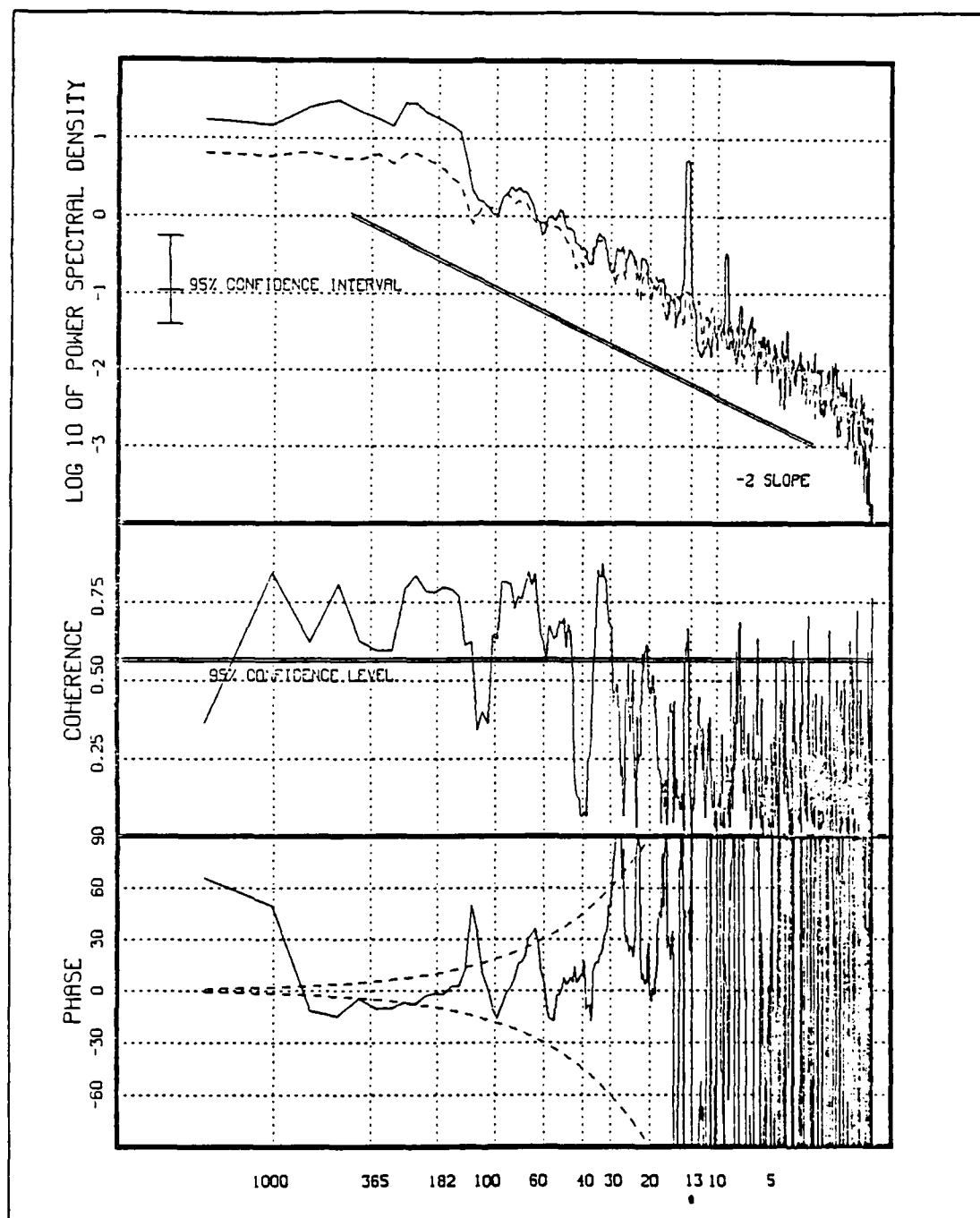
Fig. 13. Energy Density, Coherence, and Phase Spectra of \delta LOD_{USNO} and \delta LOD_{atm15} : As in Fig. 12 except the atmospheric signal is \delta LOD_{atm} computed within 15^\circ of the equator.
