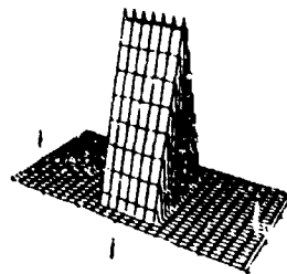
V_i^{16,1}(j)
