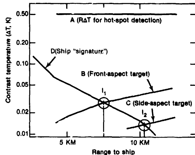
Figure 5. Acquisition range calculations for strawman seeker and target characteristics provided in Table 1.
