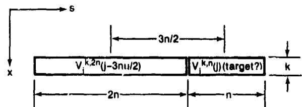
Figure 22. Image area used by low-noise background estimator, Eq. (57). Scan direction (s) is parallel to the horizon.
