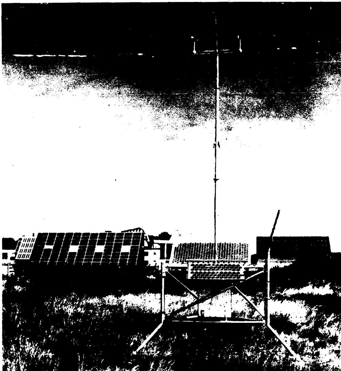
Figure II-6. FLOWS automatic weather station. Solar panels are visible above white armored box. Vane aspirator is at left (white tube with fin) and antenna is at right.
