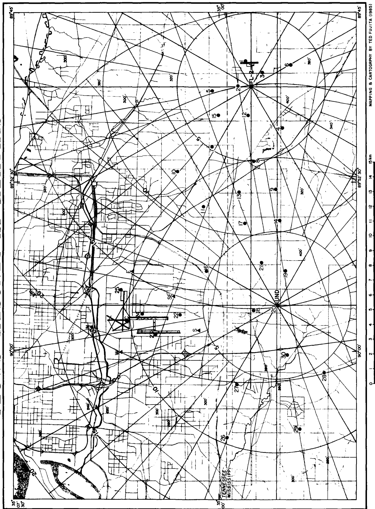
Figure II-9. 1985 FLOWS Automatic Weather Station Network.
