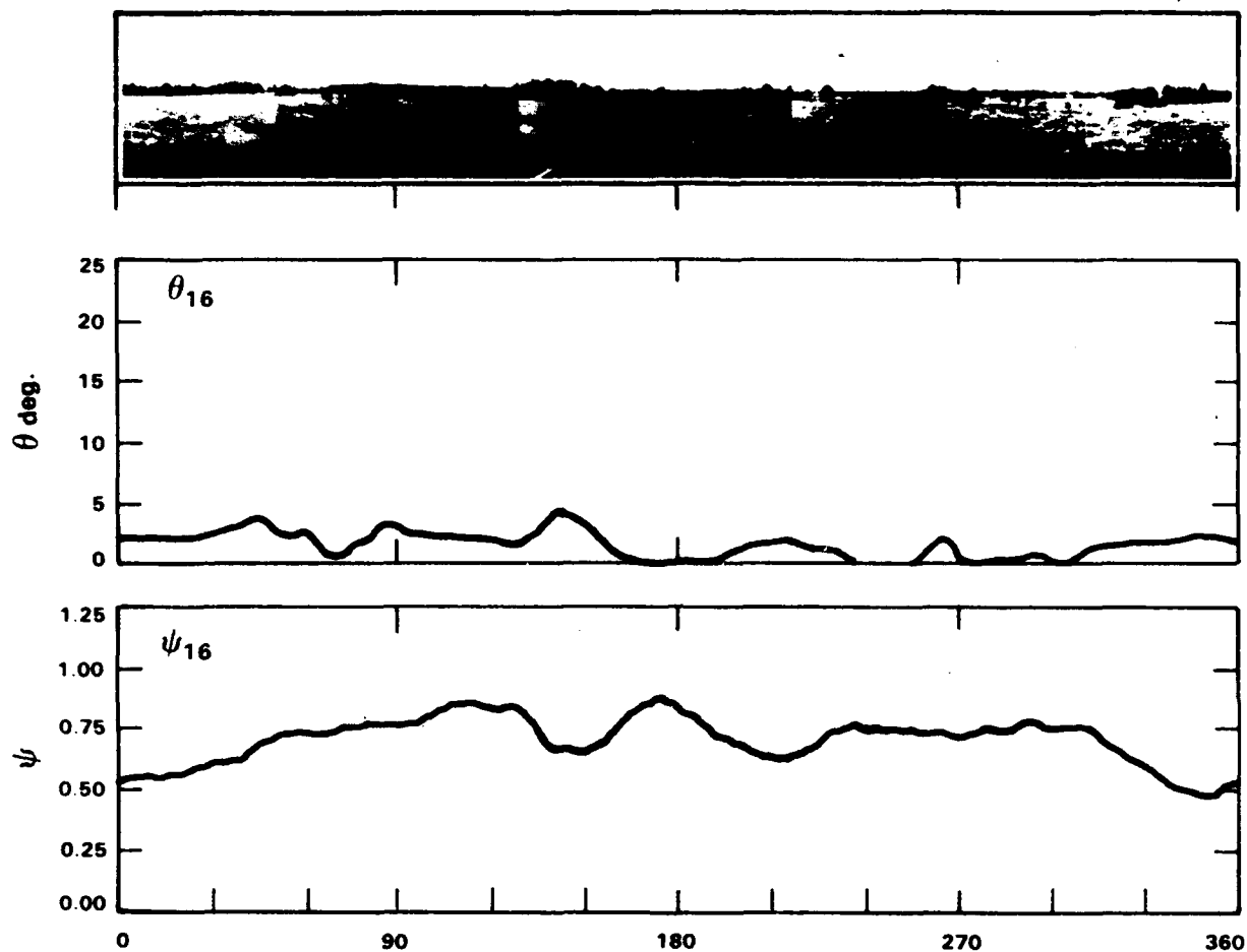
Figure V-5. Panoramic photograph, smoothed obstruction angles \theta_{16} , and smoothed transmission factors \psi_{16} for station No. 8.
