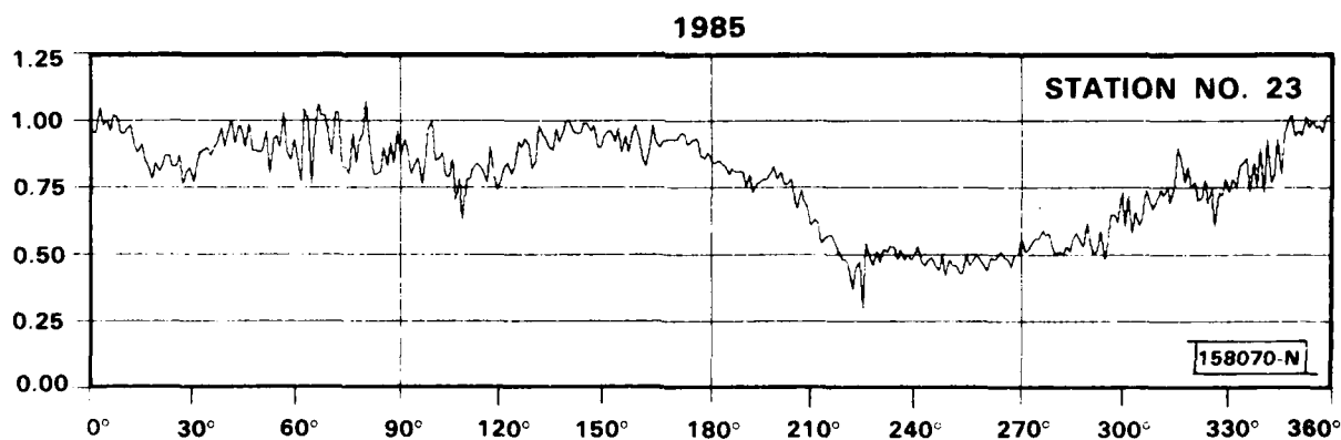
Figure IV-2. Normalized mean wind speed for station No. 23 averaged for the entire month of July 1985. Fewer winds were measured at 45°, 135°, 225° and 315° than at other azimuths and when they were measured, they were lighter than usual.
