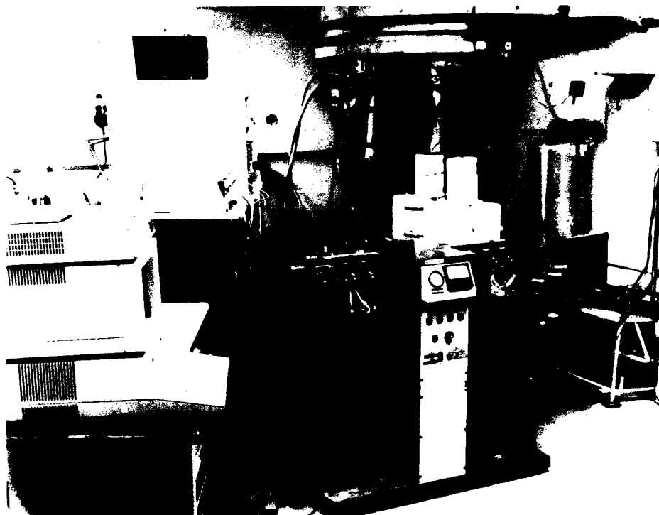
Figure III-15. View of pressure chamber, with barometers placed inside, just prior to being sealed.
