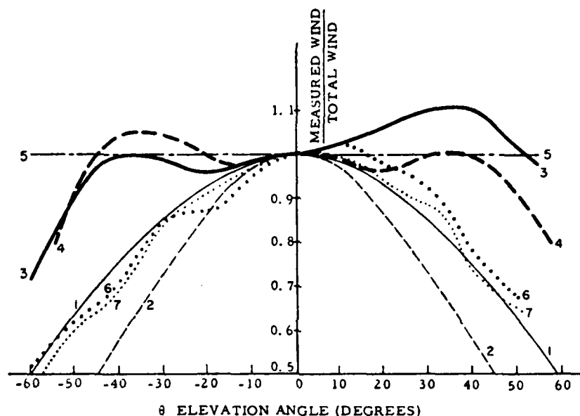
Figure III-10. Wind speed sensor sensitivity to wind elevation (flow) angle. Ratio of measured wind to total wind for various sensor responses as a function of elevation angle. Taken from MacCready (1966).
