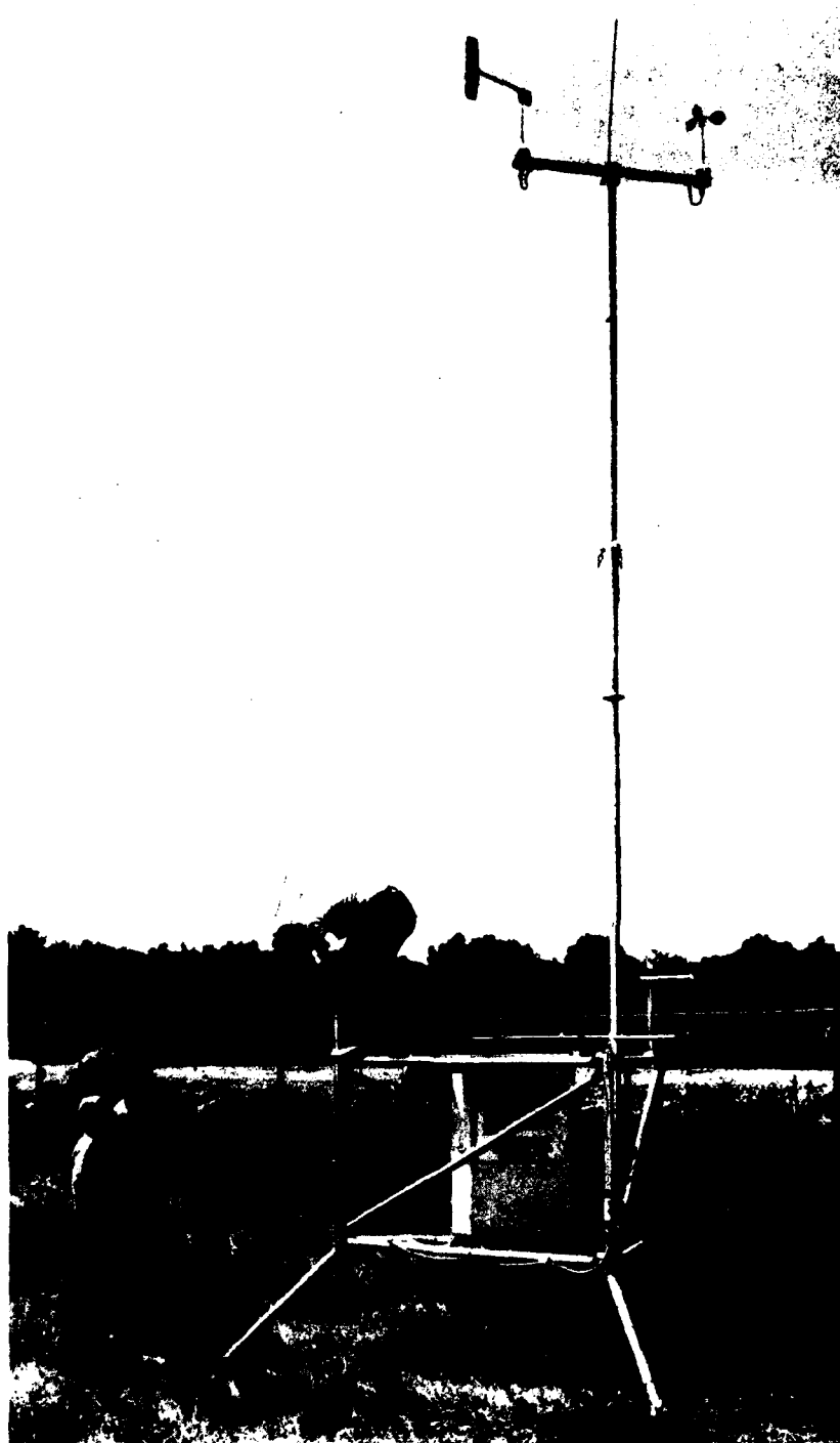
Figure II-7. View of automatic weather station features not shown in Figure II-6. Technician is working on antenna. Notice wind sensor mast is self-guyed.
