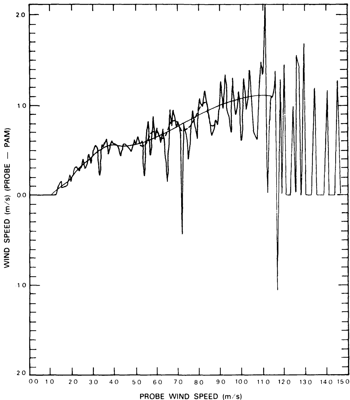
Figure III-7. Plot of wind speed difference between the PROBE (now used by Lincoln) and PAM anemometers versus PROBE wind speed. Data were collected during the 1981 CCOPE project, and show that the PROBE winds (6.8 m anemometer height) were systematically stronger than PAM winds (4.0 m anemometer height). Origins or explanations for the "spikes" in the wind discrepancies are unknown. Data provided by C. Wade at NCAR.
