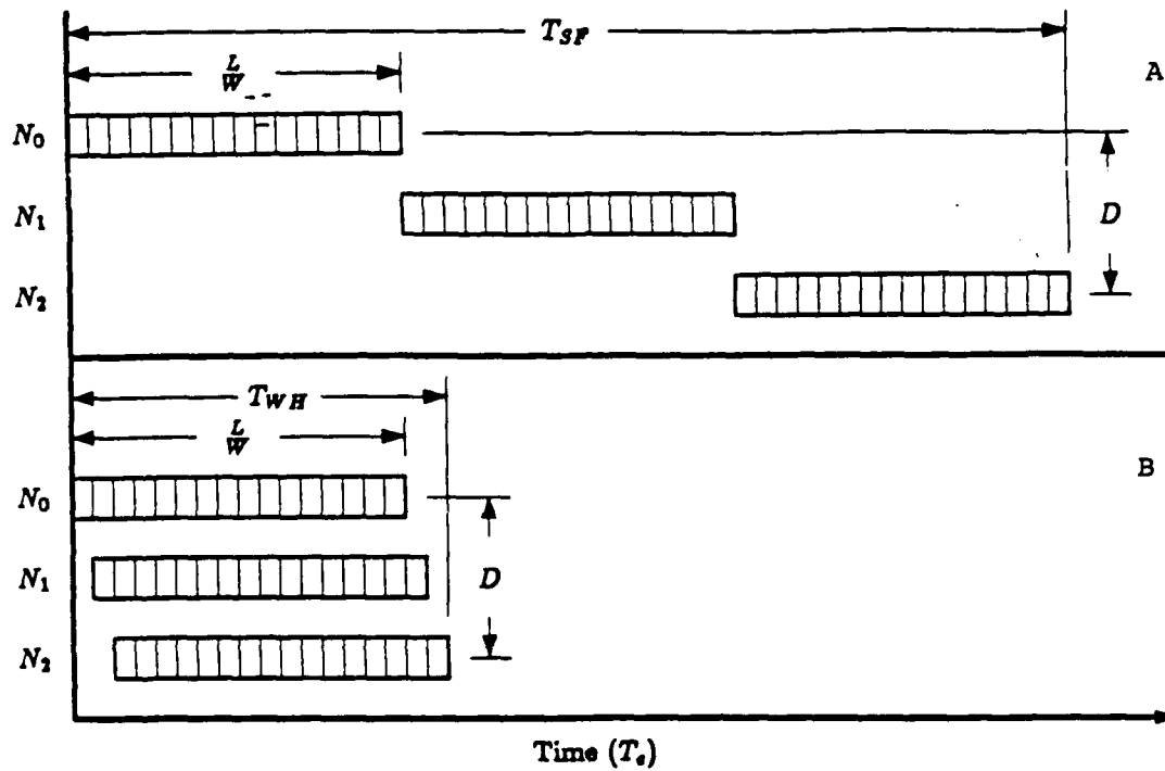
Figure 6: The latency of store-and-forward routing (A) compared to wormhole routing (B). Wormhole routing reduces latency from the product of \frac{L}{W} and D to the sum of these two components.
